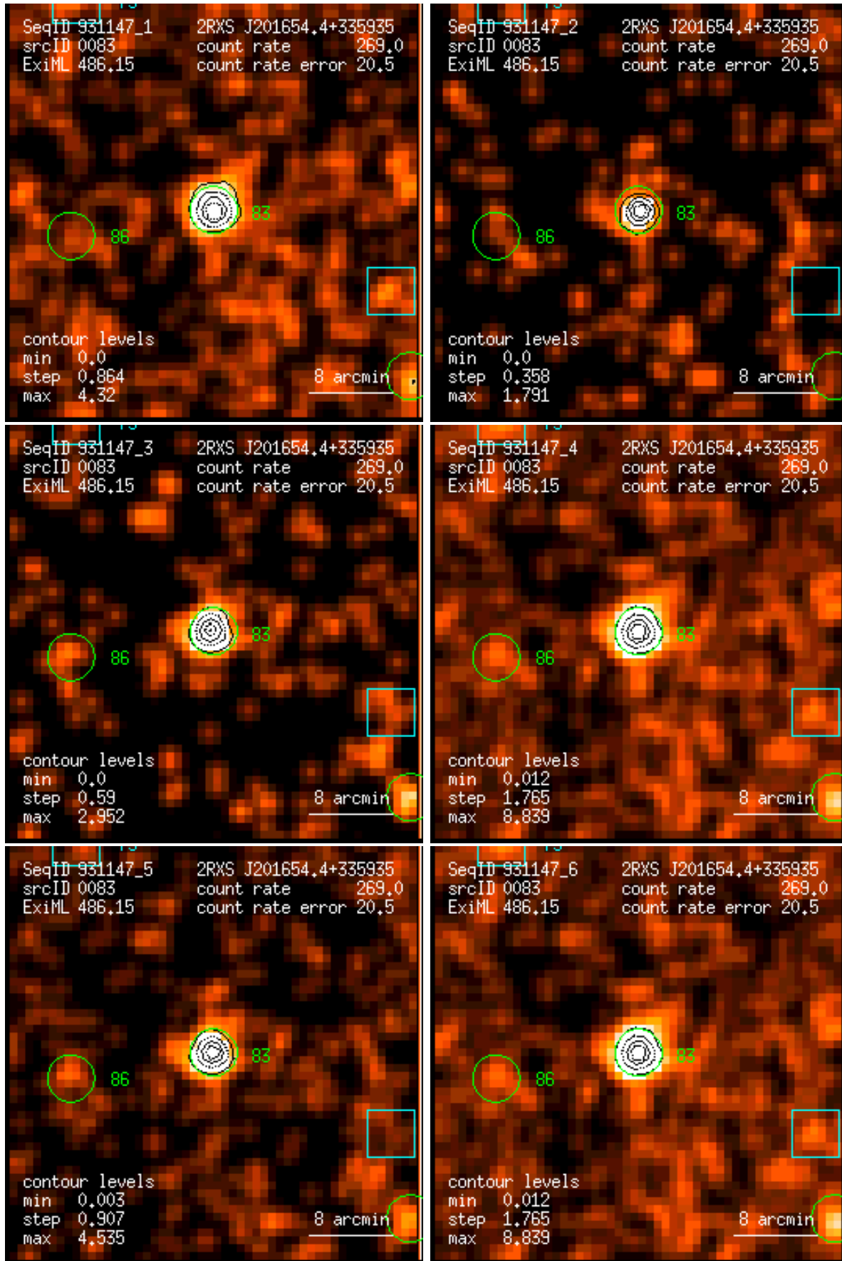
Figure 83: RASS 931147: detection 0083: band rate images, Gaussian filter: (1) PSPC channels 11 – 41, (2) 52 – 90, (3) 91 – 201, (4) 11 – 235, (5) 52 – 201, (6) 11 – 201. Broad band rates in counts/ks. Band rate contour levels in counts/ks/arcmin 2 .
