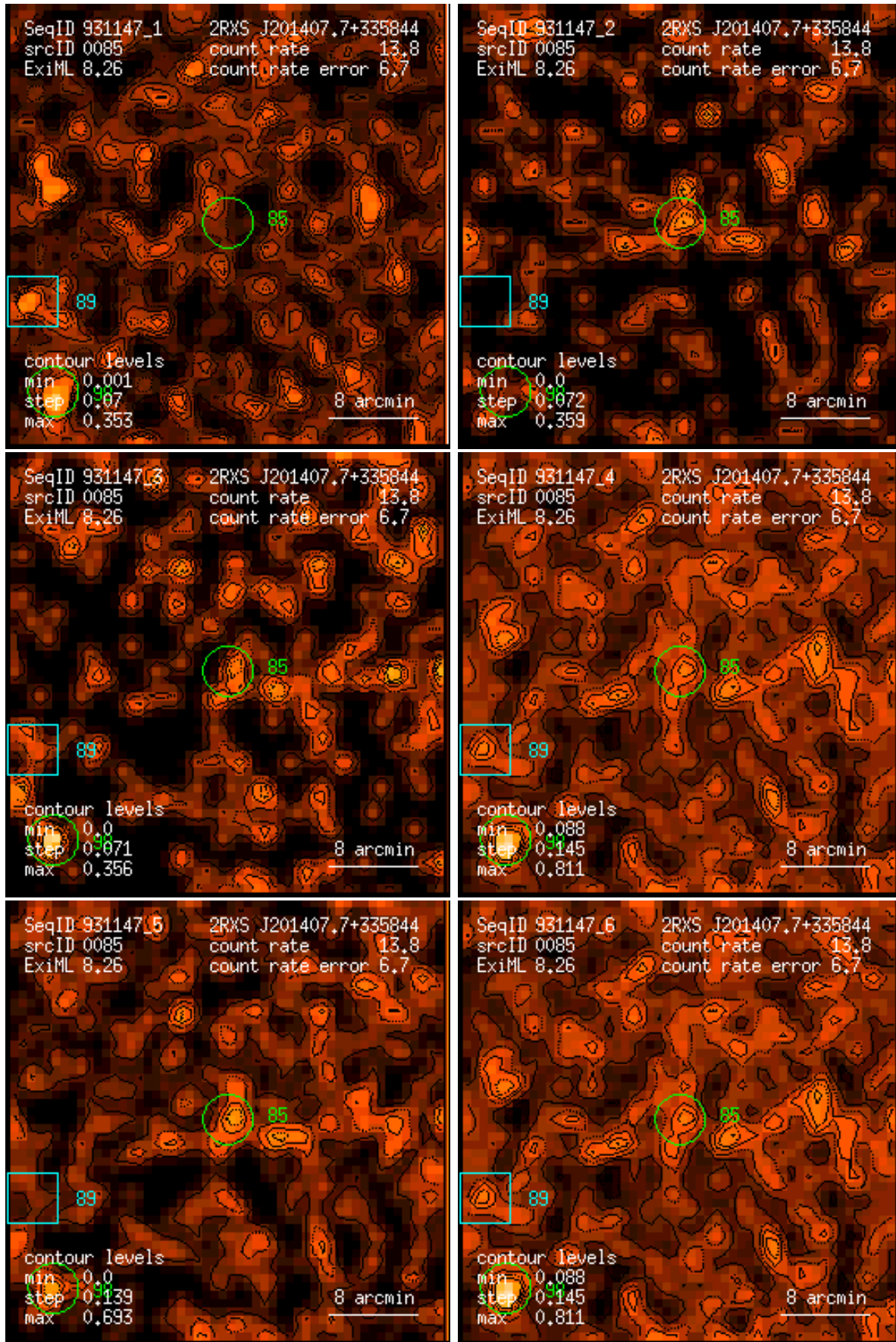
Figure 85: RASS 931147: detection 0085: band rate images, Gaussian filter: (1) PSPC channels 11 – 41, (2) 52 – 90, (3) 91 – 201, (4) 11 – 235, (5) 52 – 201, (6) 11 – 201. Broad band rates in counts/ks. Band rate contour levels in counts/ks/arcmin 2 .
