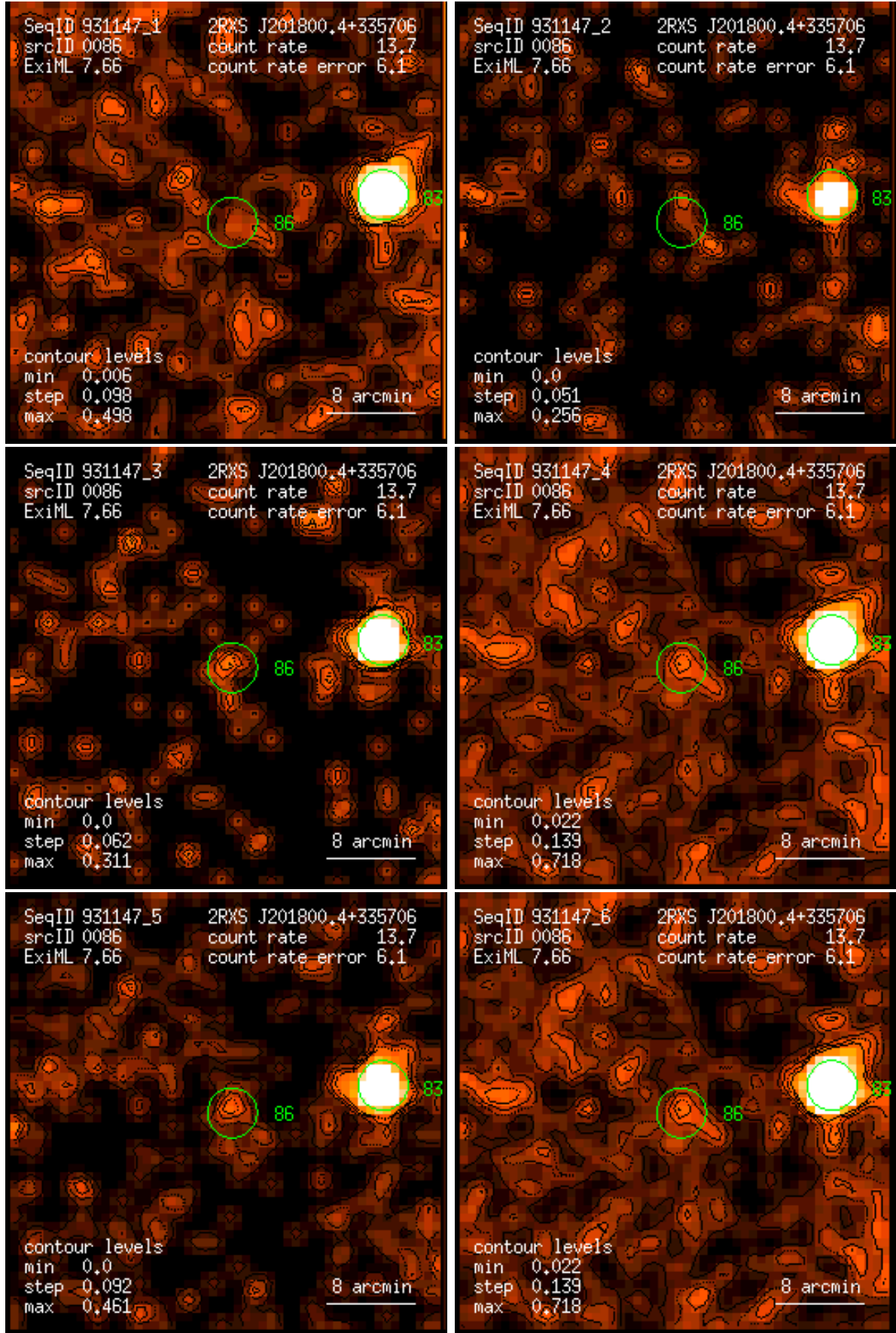
Figure 86: RASS 931147: detection 0086: band rate images, Gaussian filter: (1) PSPC channels 11 – 41, (2) 52 – 90, (3) 91 – 201, (4) 11 – 235, (5) 52 – 201, (6) 11 – 201. Broad band rates in counts/ks. Band rate contour levels in counts/ks/arcmin 2 .
