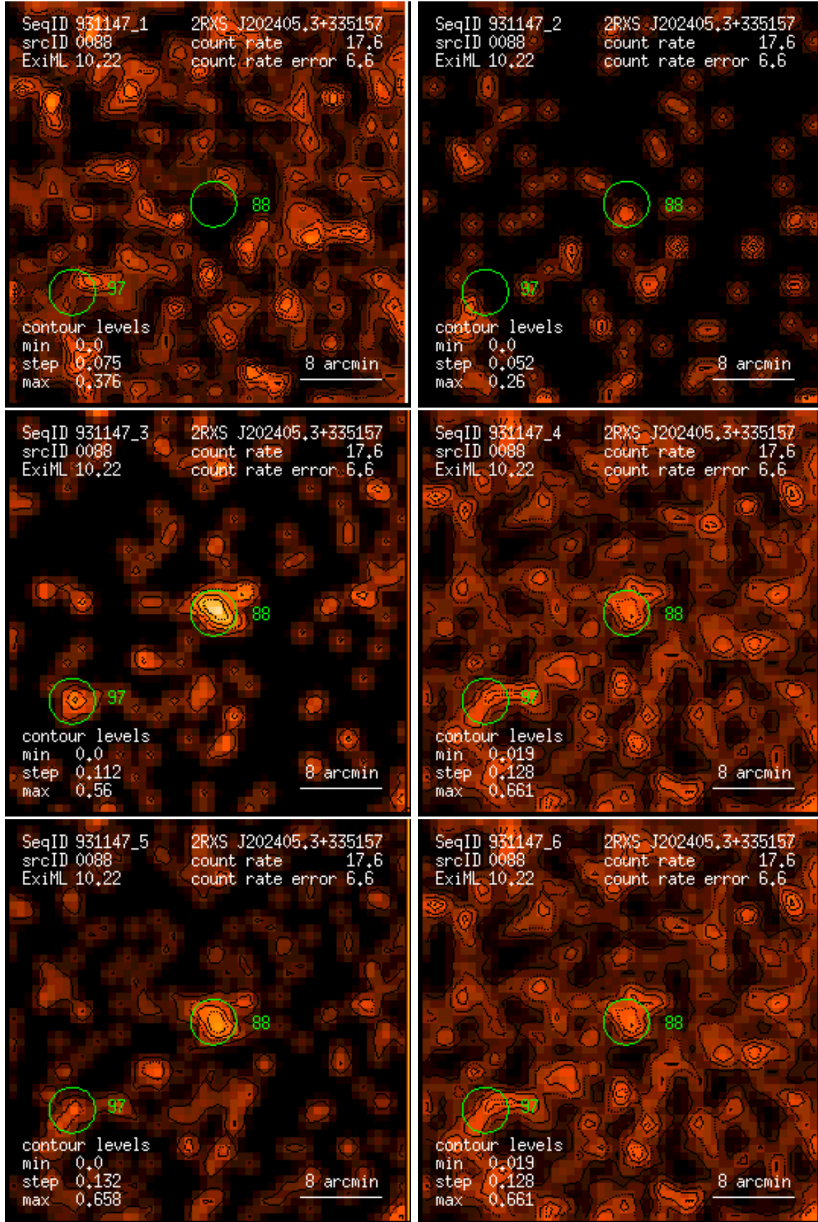
Figure 88: RASS 931147: detection 0088: band rate images, Gaussian filter: (1) PSPC channels 11 – 41, (2) 52 – 90, (3) 91 – 201, (4) 11 – 235, (5) 52 – 201, (6) 11 – 201. Broad band rates in counts/ks. Band rate contour levels in counts/ks/arcmin 2 .
