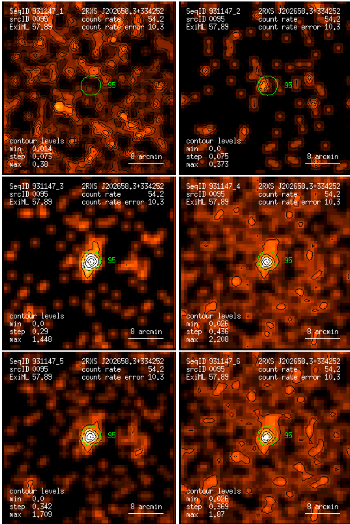
Figure 95: RASS 931147: detection 0095: band rate images, Gaussian filter: (1) PSPC channels 11 – 41, (2) 52 – 90, (3) 91 – 201, (4) 11 – 235, (5) 52 – 201, (6) 11 – 201. Broad band rates in counts/ks. Band rate contour levels in counts/ks/arcmin 2 .
