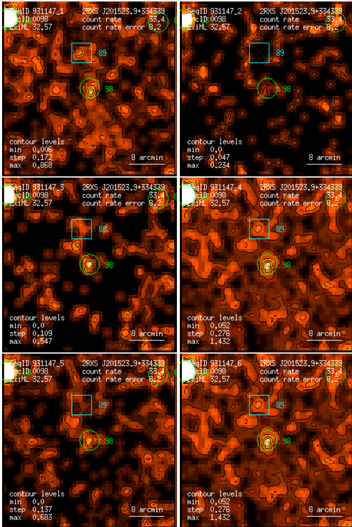
Figure 98: RASS 931147: detection 0098: band rate images, Gaussian filter: (1) PSPC channels 11 – 41, (2) 52 – 90, (3) 91 – 201, (4) 11 – 235, (5) 52 – 201, (6) 11 – 201. Broad band rates in counts/ks. Band rate contour levels in counts/ks/arcmin 2 .
