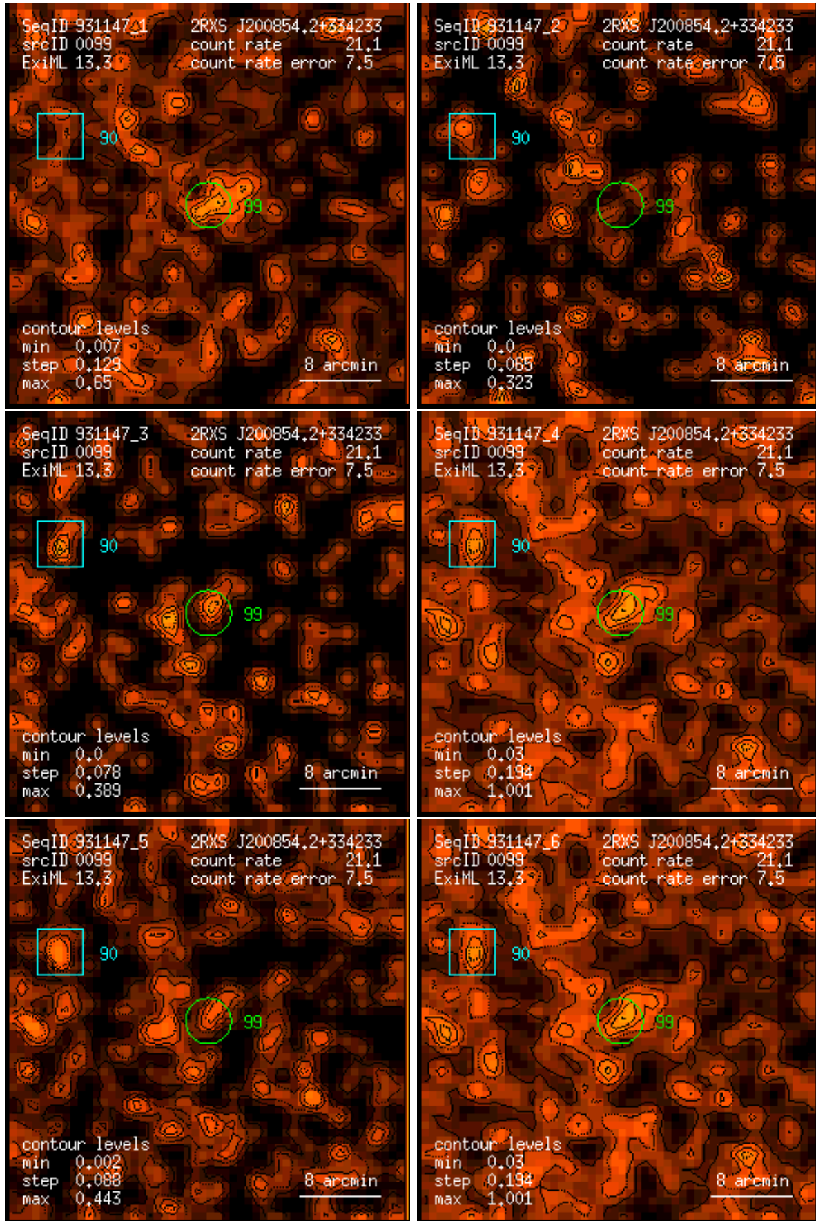
Figure 99: RASS 931147: detection 0099: band rate images, Gaussian filter: (1) PSPC channels 11 – 41, (2) 52 – 90, (3) 91 – 201, (4) 11 – 235, (5) 52 – 201, (6) 11 – 201. Broad band rates in counts/ks. Band rate contour levels in counts/ks/arcmin 2 .
