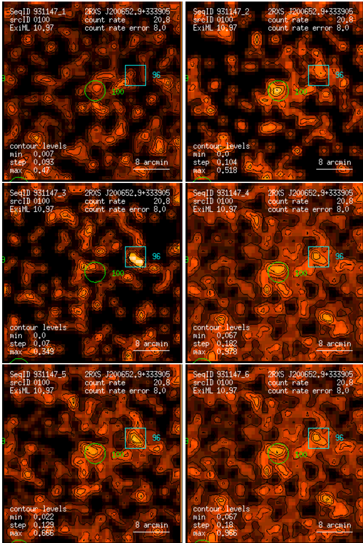
Figure 100: RASS 931147: detection 0100: band rate images, Gaussian filter: (1) PSPC channels 11 – 41, (2) 52 – 90, (3) 91 – 201, (4) 11 – 235, (5) 52 – 201, (6) 11 – 201. Broad band rates in counts/ks. Band rate contour levels in counts/ks/arcmin 2 .
