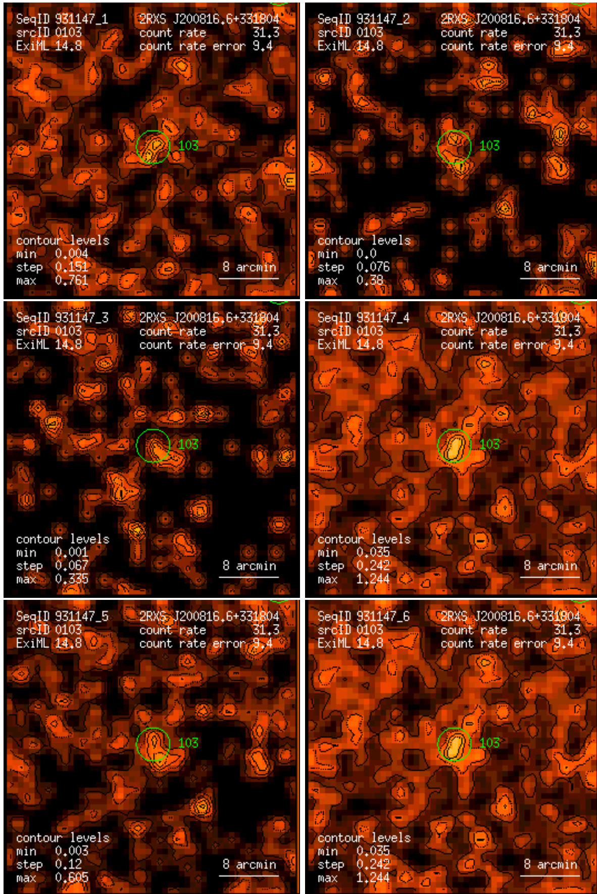
Figure 103: RASS 931147: detection 0103: band rate images, Gaussian filter: (1) PSPC channels 11 – 41, (2) 52 – 90, (3) 91 – 201, (4) 11 – 235, (5) 52 – 201, (6) 11 – 201. Broad band rates in counts/ks. Band rate contour levels in counts/ks/arcmin 2 .
