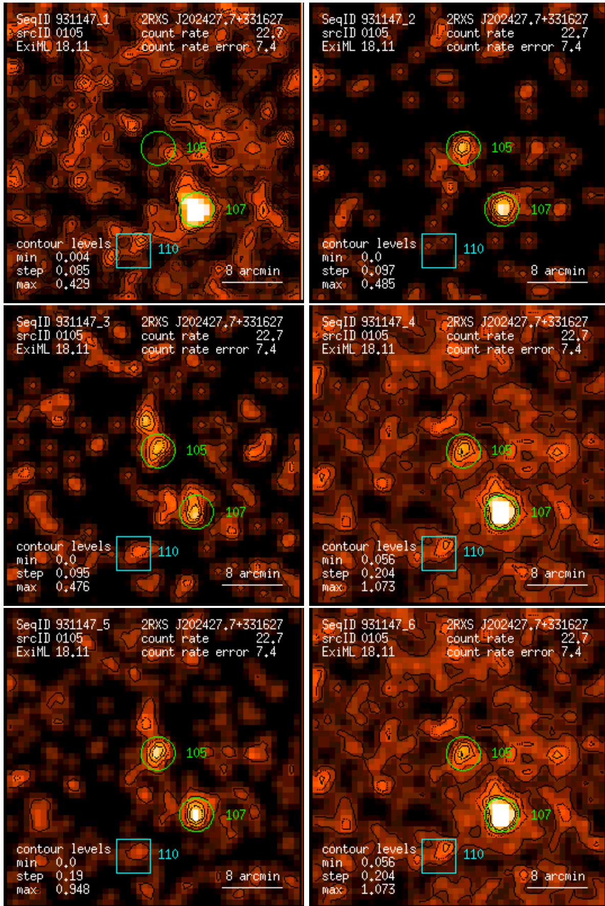
Figure 105: RASS 931147: detection 0105: band rate images, Gaussian filter: (1) PSPC channels 11 – 41, (2) 52 – 90, (3) 91 – 201, (4) 11 – 235, (5) 52 – 201, (6) 11 – 201. Broad band rates in counts/ks. Band rate contour levels in counts/ks/arcmin 2 .
