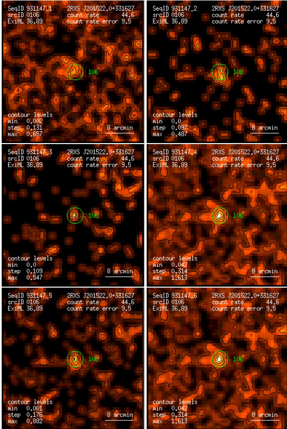
Figure 106: RASS 931147: detection 0106: band rate images, Gaussian filter: (1) PSPC channels 11 – 41, (2) 52 – 90, (3) 91 – 201, (4) 11 – 235, (5) 52 – 201, (6) 11 – 201. Broad band rates in counts/ks. Band rate contour levels in counts/ks/arcmin 2 .
