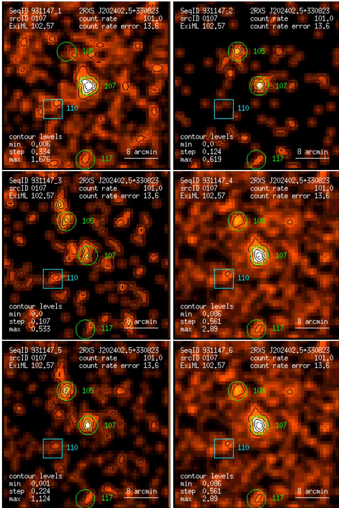
Figure 107: RASS 931147: detection 0107: band rate images, Gaussian filter: (1) PSPC channels 11 – 41, (2) 52 – 90, (3) 91 – 201, (4) 11 – 235, (5) 52 – 201, (6) 11 – 201. Broad band rates in counts/ks. Band rate contour levels in counts/ks/arcmin 2 .
