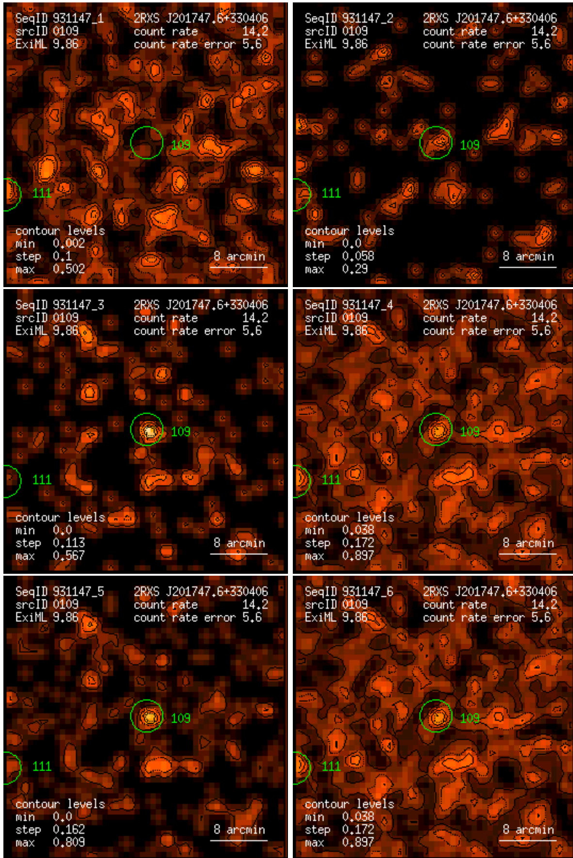
Figure 109: RASS 931147: detection 0109: band rate images, Gaussian filter: (1) PSPC channels 11 – 41, (2) 52 – 90, (3) 91 – 201, (4) 11 – 235, (5) 52 – 201, (6) 11 – 201. Broad band rates in counts/ks. Band rate contour levels in counts/ks/arcmin 2 .
