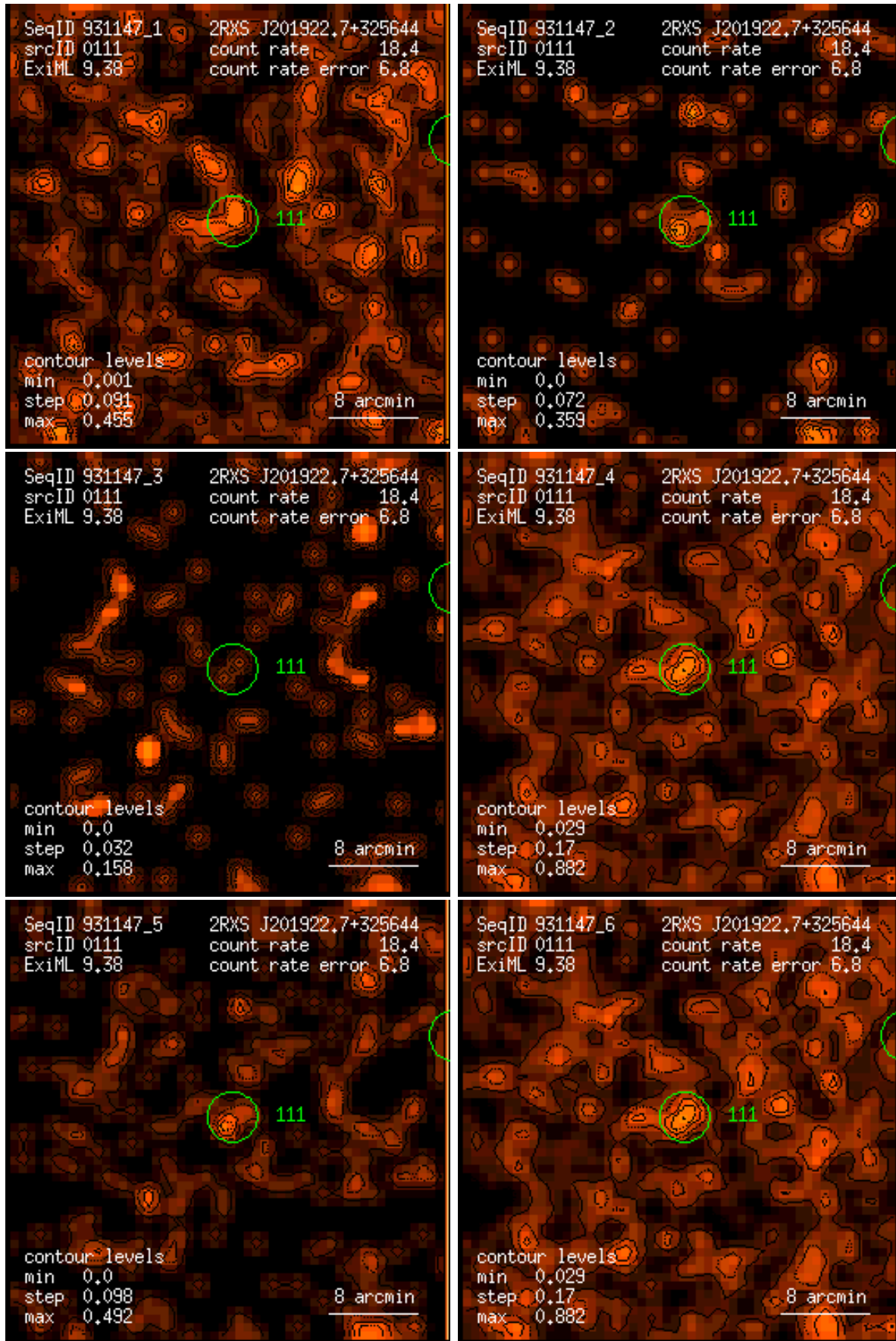
Figure 111: RASS 931147: detection 0111: band rate images, Gaussian filter: (1) PSPC channels 11 – 41, (2) 52 – 90, (3) 91 – 201, (4) 11 – 235, (5) 52 – 201, (6) 11 – 201. Broad band rates in counts/ks. Band rate contour levels in counts/ks/arcmin 2 .
