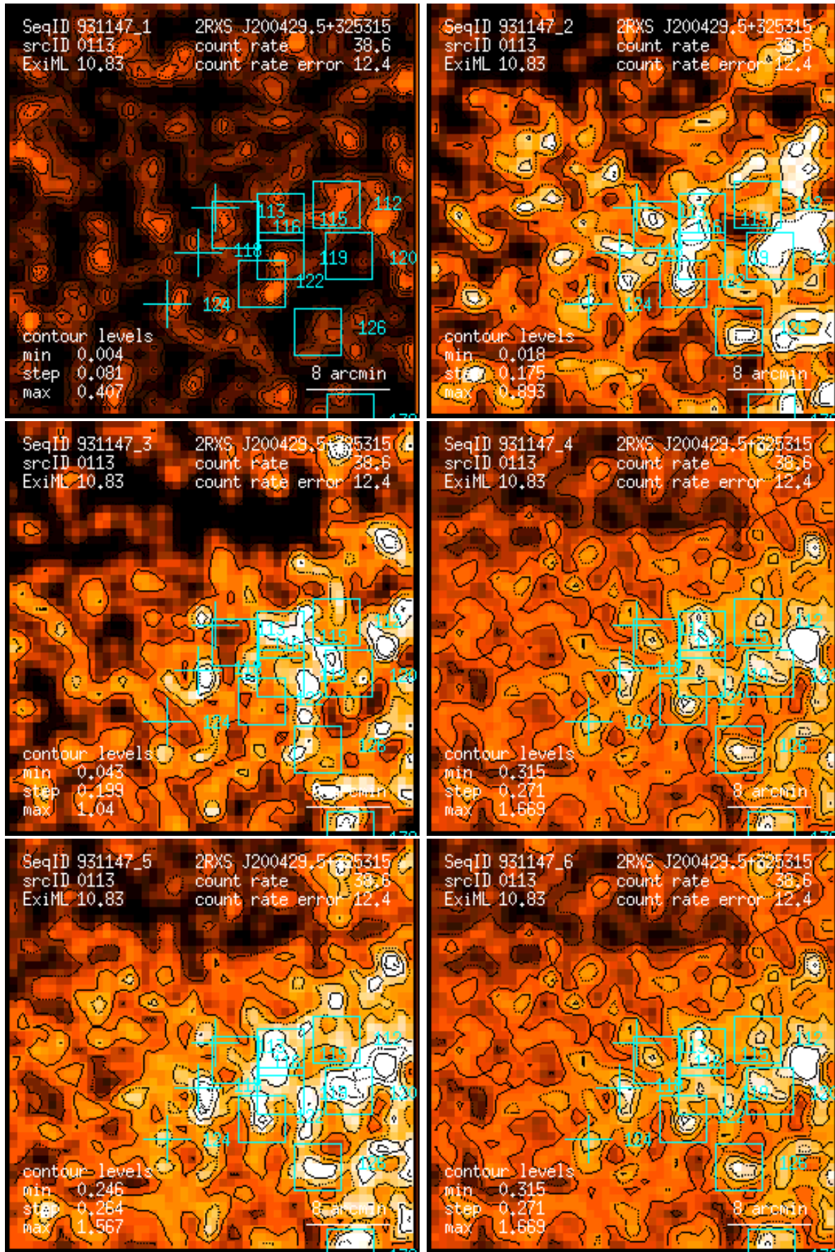
Figure 113: RASS 931147: detection 0113: band rate images, Gaussian filter: (1) PSPC channels 11 – 41, (2) 52 – 90, (3) 91 – 201, (4) 11 – 235, (5) 52 – 201, (6) 11 – 201. Broad band rates in counts/ks. Band rate contour levels in counts/ks/arcmin 2 .
