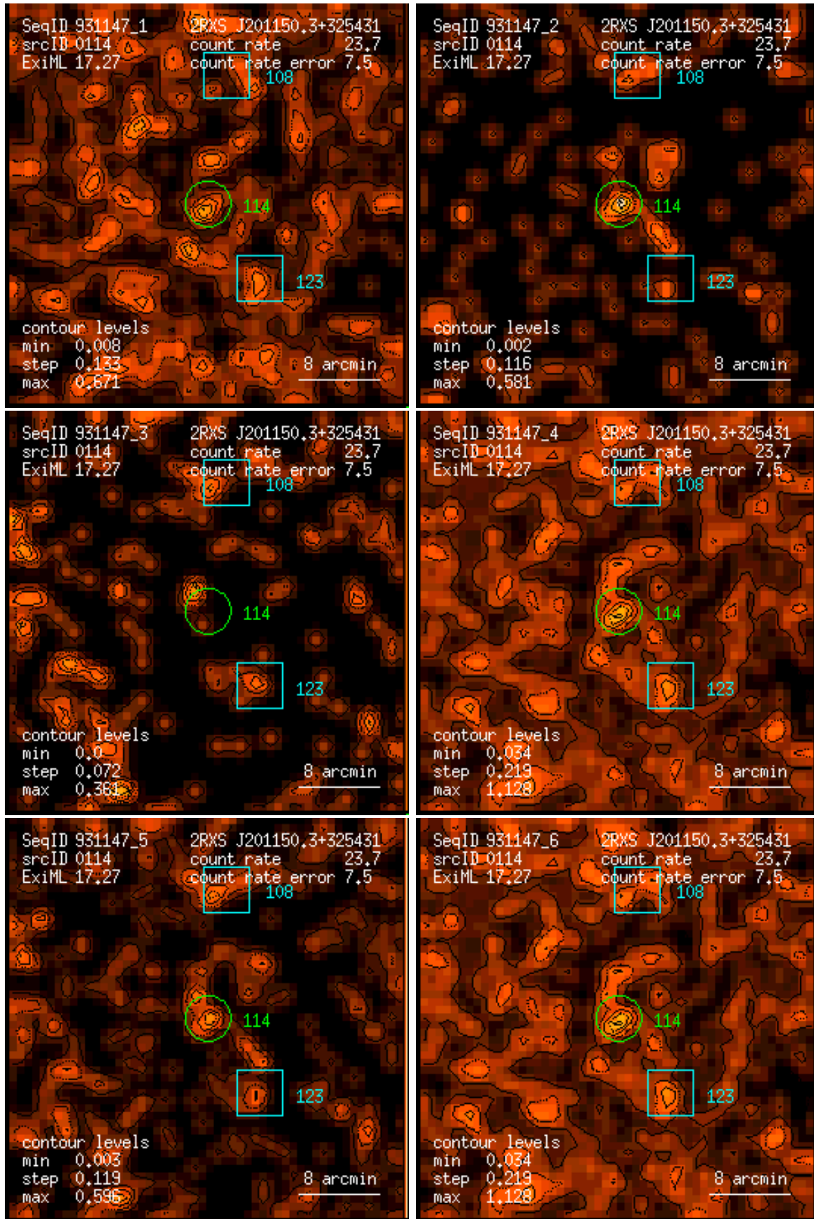
Figure 114: RASS 931147: detection 0114: band rate images, Gaussian filter: (1) PSPC channels 11 – 41, (2) 52 – 90, (3) 91 – 201, (4) 11 – 235, (5) 52 – 201, (6) 11 – 201. Broad band rates in counts/ks. Band rate contour levels in counts/ks/arcmin 2 .
