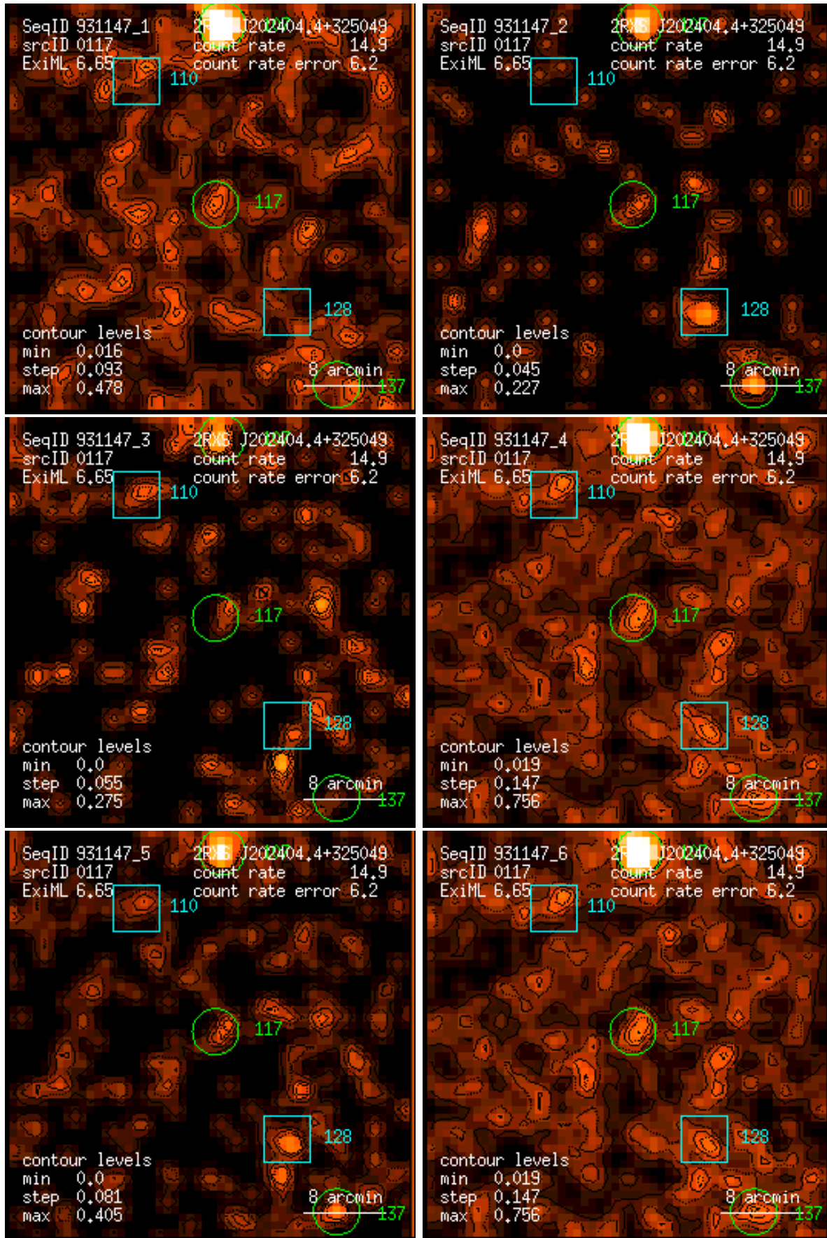
Figure 117: RASS 931147: detection 0117: band rate images, Gaussian filter: (1) PSPC channels 11 – 41, (2) 52 – 90, (3) 91 – 201, (4) 11 – 235, (5) 52 – 201, (6) 11 – 201. Broad band rates in counts/ks. Band rate contour levels in counts/ks/arcmin 2 .
