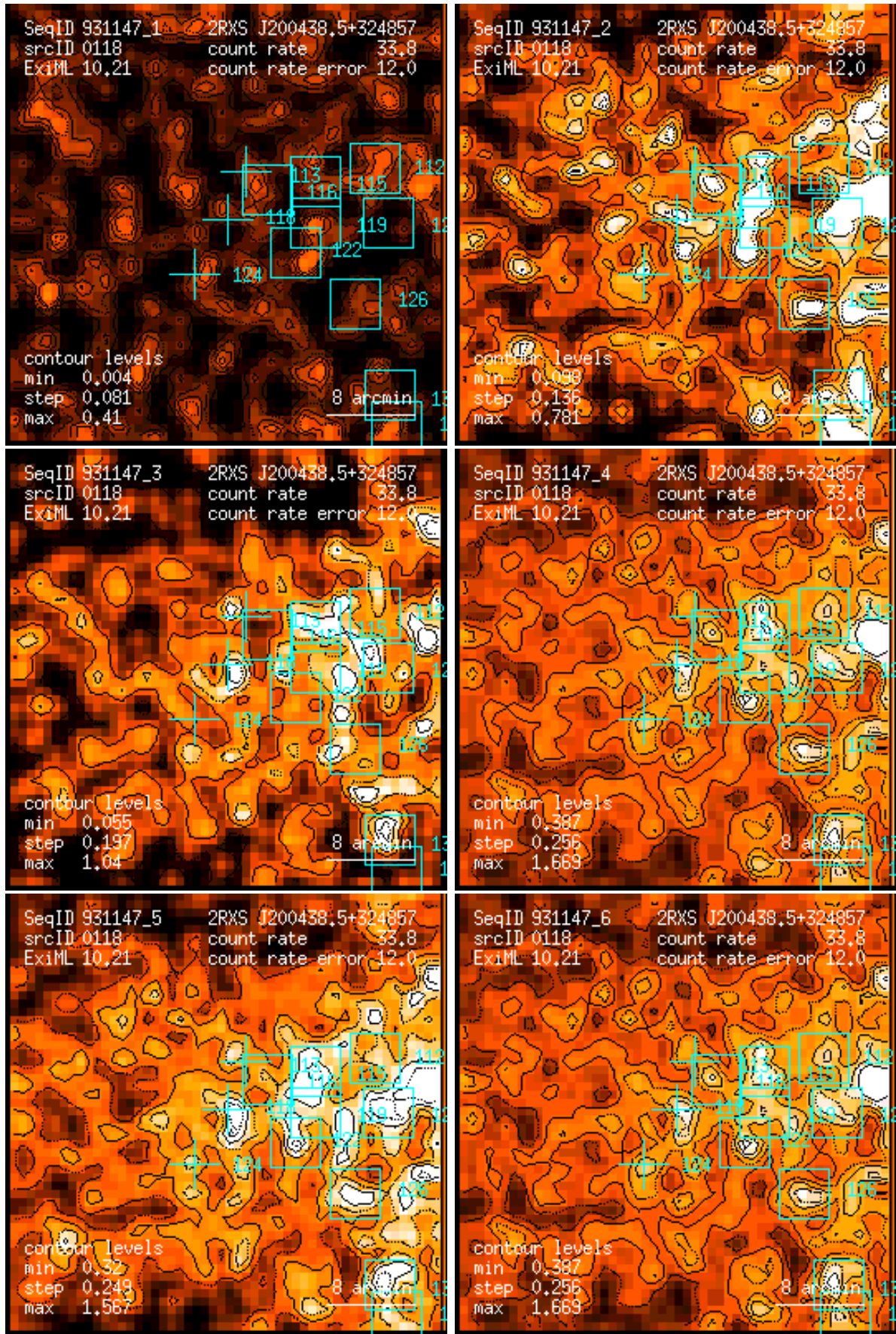
Figure 118: RASS 931147: detection 0118: band rate images, Gaussian filter: (1) PSPC channels 11 – 41, (2) 52 – 90, (3) 91 – 201, (4) 11 – 235, (5) 52 – 201, (6) 11 – 201. Broad band rates in counts/ks. Band rate contour levels in counts/ks/arcmin 2 .
