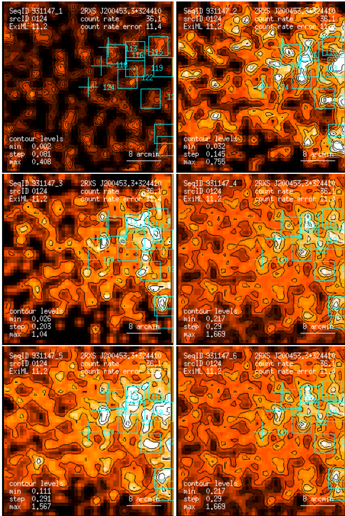
Figure 124: RASS 931147: detection 0124: band rate images, Gaussian filter: (1) PSPC channels 11 – 41, (2) 52 – 90, (3) 91 – 201, (4) 11 – 235, (5) 52 – 201, (6) 11 – 201. Broad band rates in counts/ks. Band rate contour levels in counts/ks/arcmin 2 .
