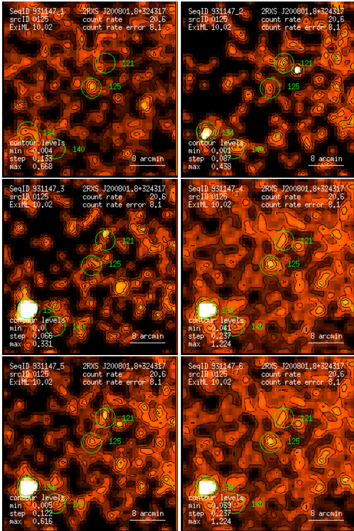
Figure 125: RASS 931147: detection 0125: band rate images, Gaussian filter: (1) PSPC channels 11 – 41, (2) 52 – 90, (3) 91 – 201, (4) 11 – 235, (5) 52 – 201, (6) 11 – 201. Broad band rates in counts/ks. Band rate contour levels in counts/ks/arcmin 2 .
