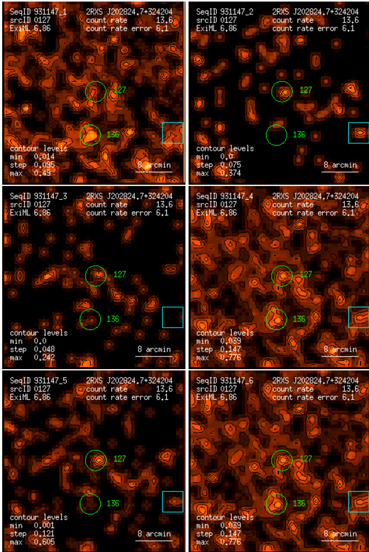
Figure 127: RASS 931147: detection 0127: band rate images, Gaussian filter: (1) PSPC channels 11 – 41, (2) 52 – 90, (3) 91 – 201, (4) 11 – 235, (5) 52 – 201, (6) 11 – 201. Broad band rates in counts/ks. Band rate contour levels in counts/ks/arcmin 2 .
