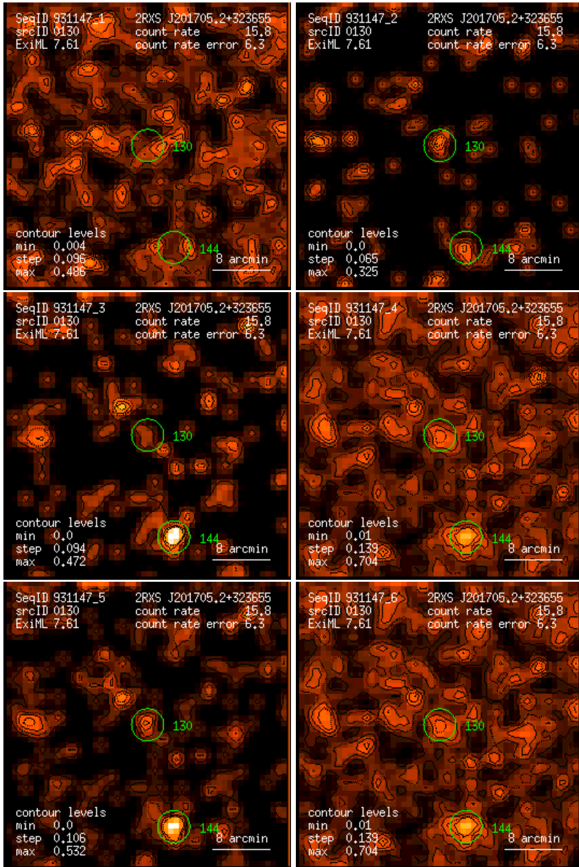
Figure 130: RASS 931147: detection 0130: band rate images, Gaussian filter: (1) PSPC channels 11 – 41, (2) 52 – 90, (3) 91 – 201, (4) 11 – 235, (5) 52 – 201, (6) 11 – 201. Broad band rates in counts/ks. Band rate contour levels in counts/ks/arcmin 2 .
