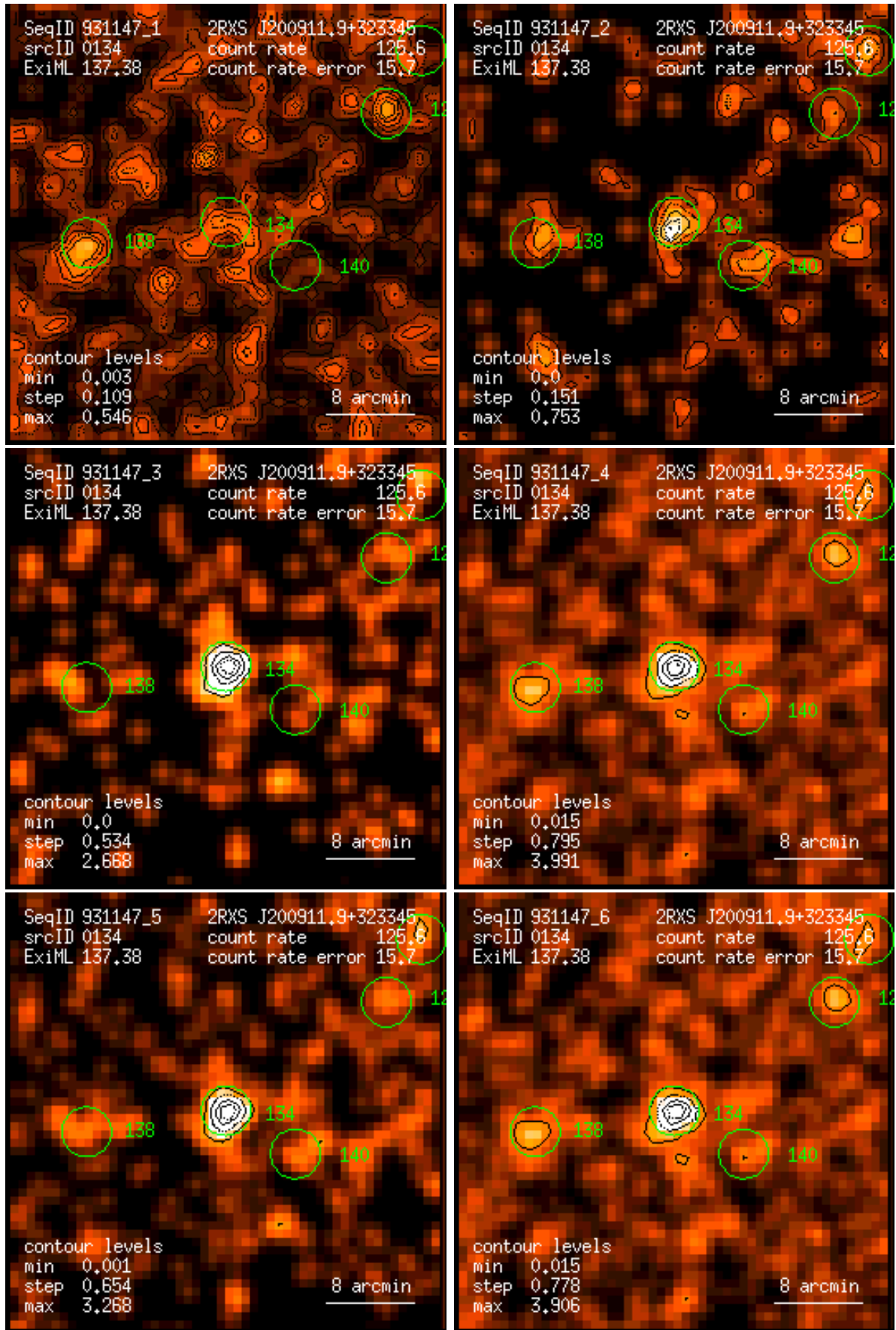
Figure 134: RASS 931147: detection 0134: band rate images, Gaussian filter: (1) PSPC channels 11 – 41, (2) 52 – 90, (3) 91 – 201, (4) 11 – 235, (5) 52 – 201, (6) 11 – 201. Broad band rates in counts/ks. Band rate contour levels in counts/ks/arcmin 2 .
