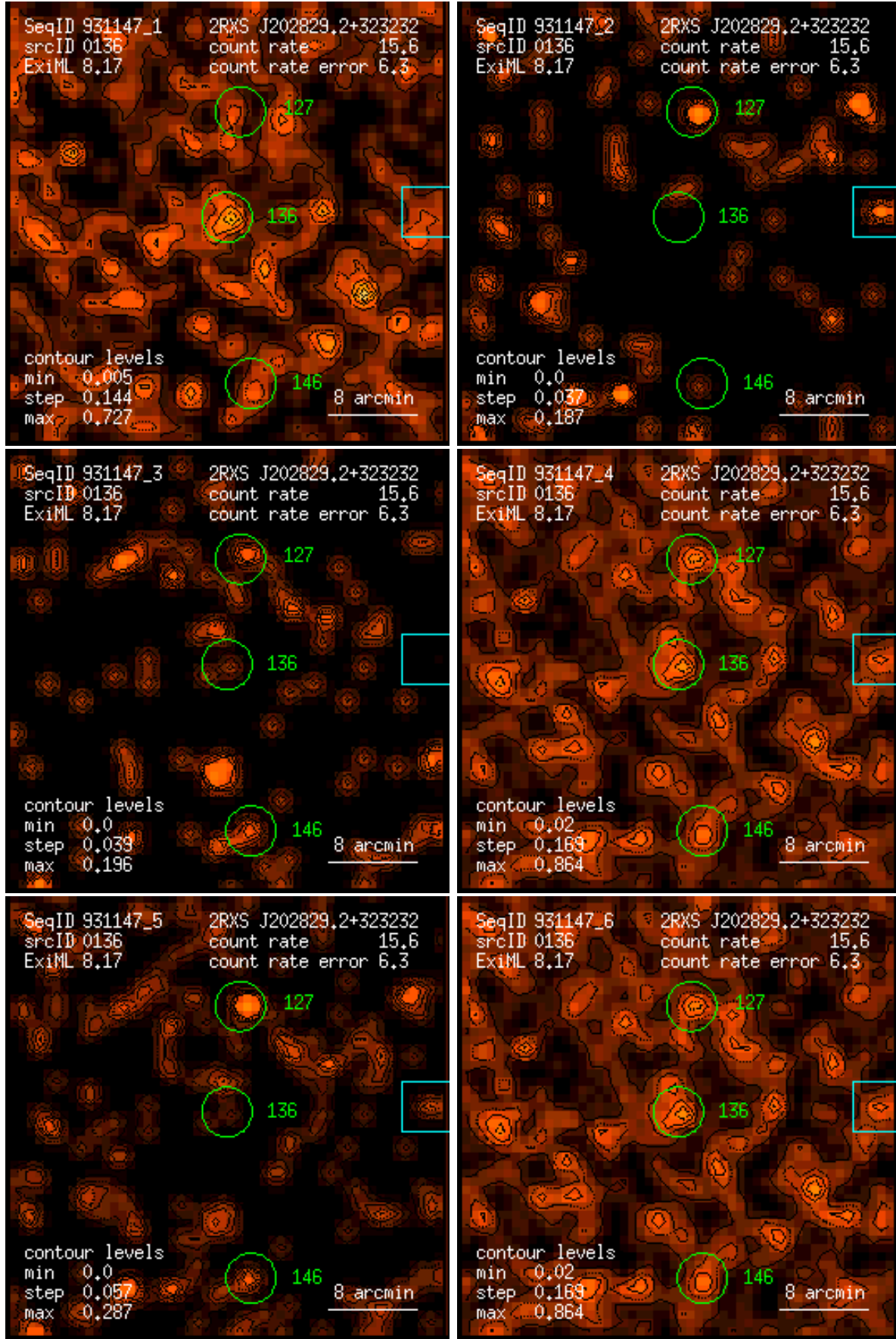
Figure 136: RASS 931147: detection 0136: band rate images, Gaussian filter: (1) PSPC channels 11 – 41, (2) 52 – 90, (3) 91 – 201, (4) 11 – 235, (5) 52 – 201, (6) 11 – 201. Broad band rates in counts/ks. Band rate contour levels in counts/ks/arcmin 2 .
