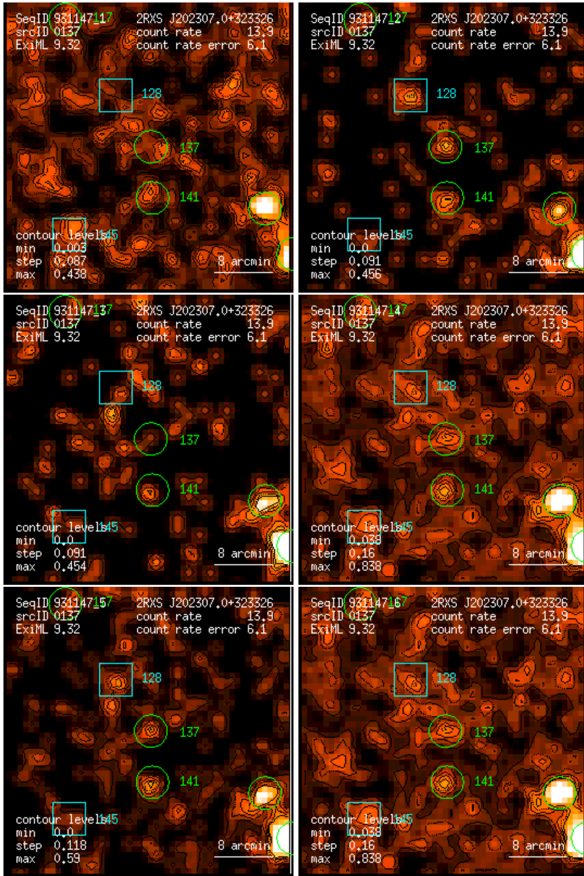
Figure 137: RASS 931147: detection 0137: band rate images, Gaussian filter: (1) PSPC channels 11 – 41, (2) 52 – 90, (3) 91 – 201, (4) 11 – 235, (5) 52 – 201, (6) 11 – 201. Broad band rates in counts/ks. Band rate contour levels in counts/ks/arcmin 2 .
