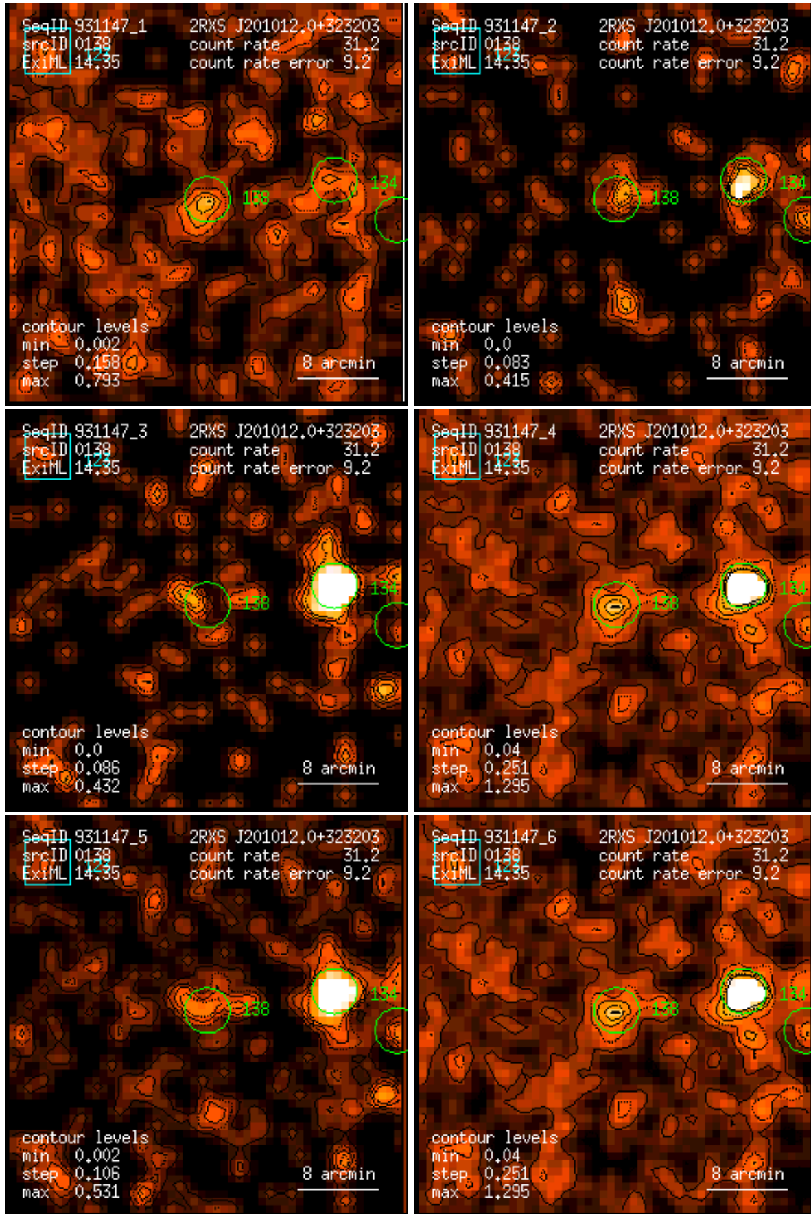
Figure 138: RASS 931147: detection 0138: band rate images, Gaussian filter: (1) PSPC channels 11 – 41, (2) 52 – 90, (3) 91 – 201, (4) 11 – 235, (5) 52 – 201, (6) 11 – 201. Broad band rates in counts/ks. Band rate contour levels in counts/ks/arcmin 2 .
