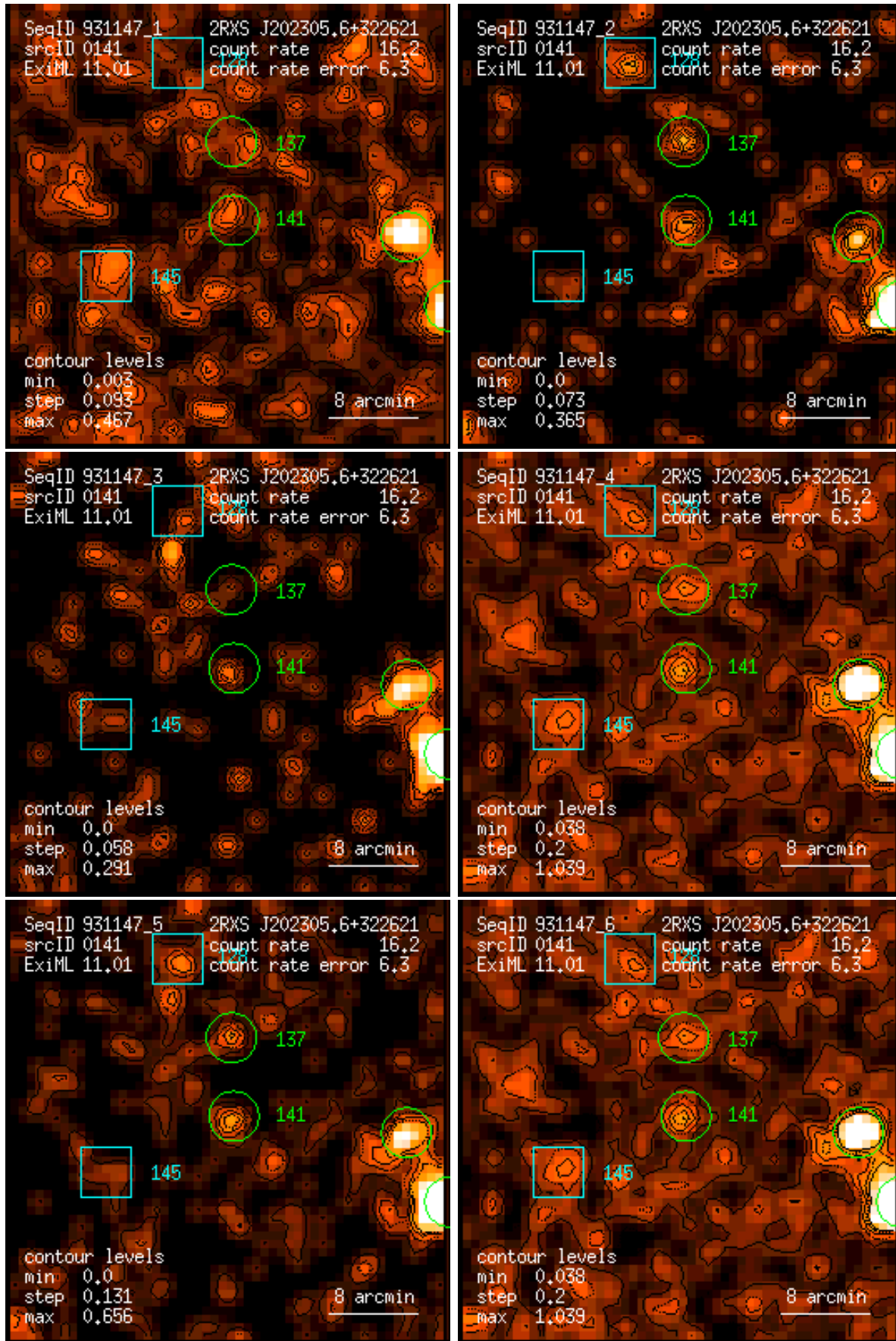
Figure 141: RASS 931147: detection 0141: band rate images, Gaussian filter: (1) PSPC channels 11 – 41, (2) 52 – 90, (3) 91 – 201, (4) 11 – 235, (5) 52 – 201, (6) 11 – 201. Broad band rates in counts/ks. Band rate contour levels in counts/ks/arcmin 2 .
