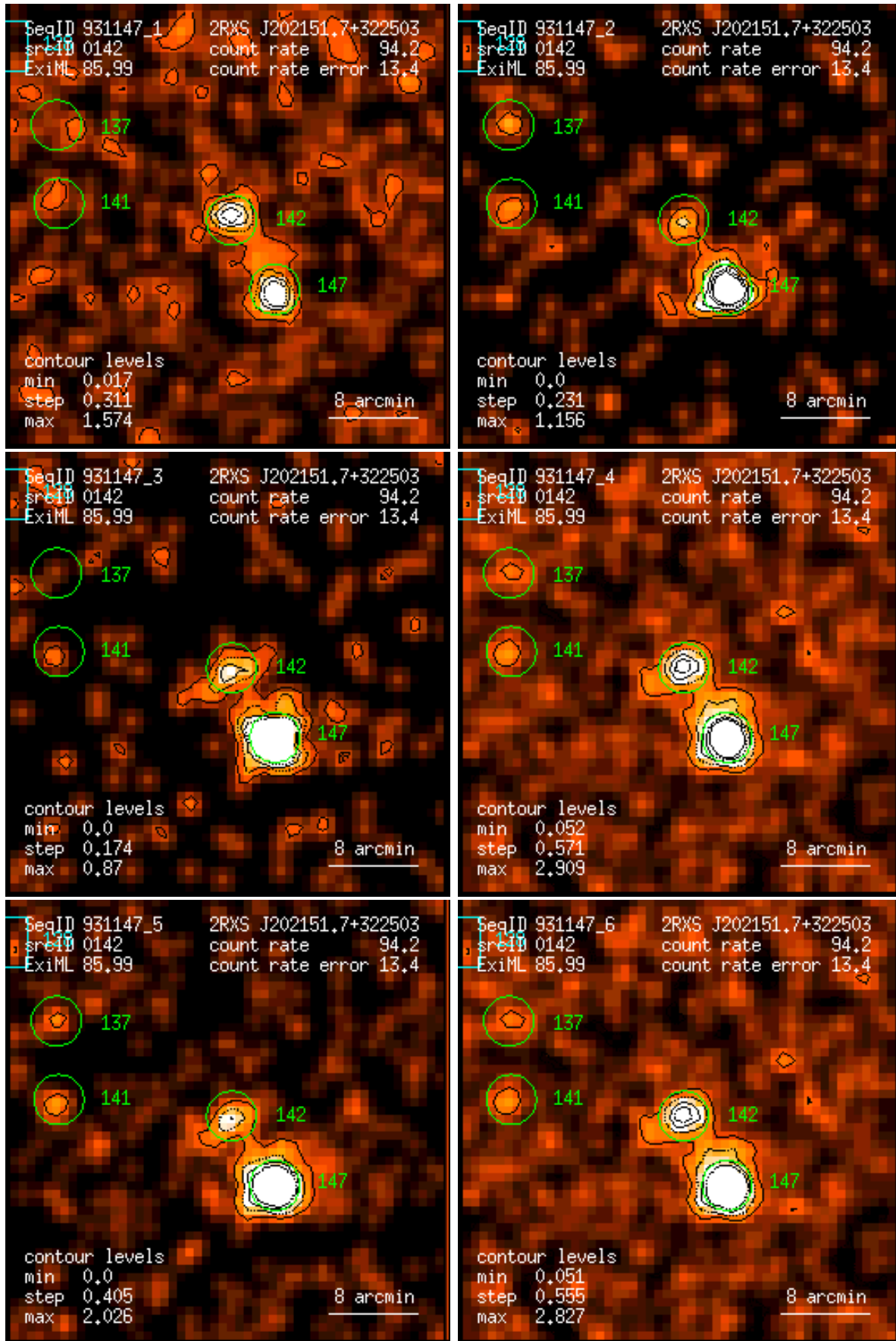
Figure 142: RASS 931147: detection 0142: band rate images, Gaussian filter: (1) PSPC channels 11 – 41, (2) 52 – 90, (3) 91 – 201, (4) 11 – 235, (5) 52 – 201, (6) 11 – 201. Broad band rates in counts/ks. Band rate contour levels in counts/ks/arcmin 2 .
