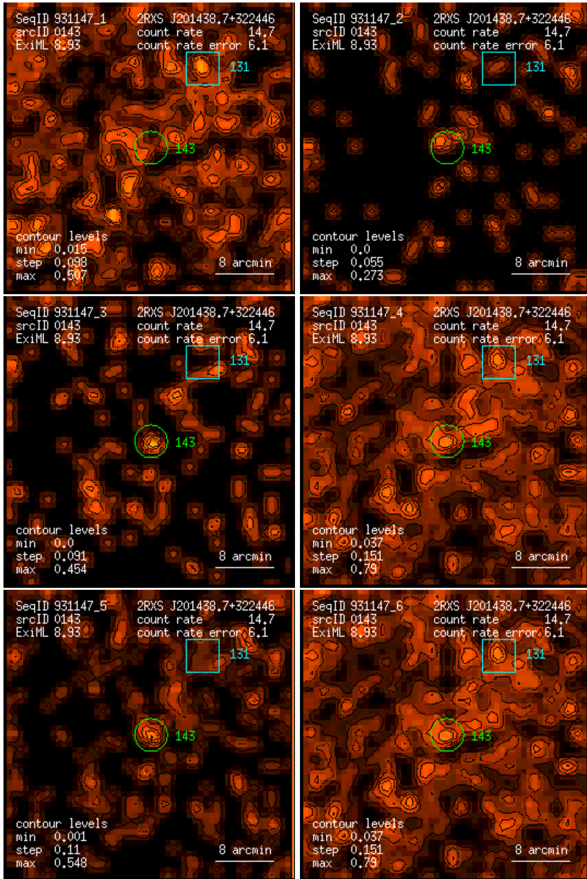
Figure 143: RASS 931147: detection 0143: band rate images, Gaussian filter: (1) PSPC channels 11 – 41, (2) 52 – 90, (3) 91 – 201, (4) 11 – 235, (5) 52 – 201, (6) 11 – 201. Broad band rates in counts/ks. Band rate contour levels in counts/ks/arcmin 2 .
