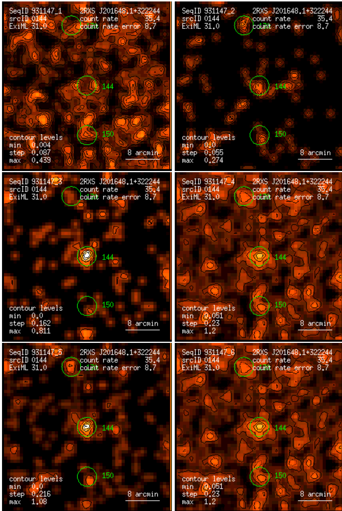
Figure 144: RASS 931147: detection 0144: band rate images, Gaussian filter: (1) PSPC channels 11 – 41, (2) 52 – 90, (3) 91 – 201, (4) 11 – 235, (5) 52 – 201, (6) 11 – 201. Broad band rates in counts/ks. Band rate contour levels in counts/ks/arcmin 2 .
