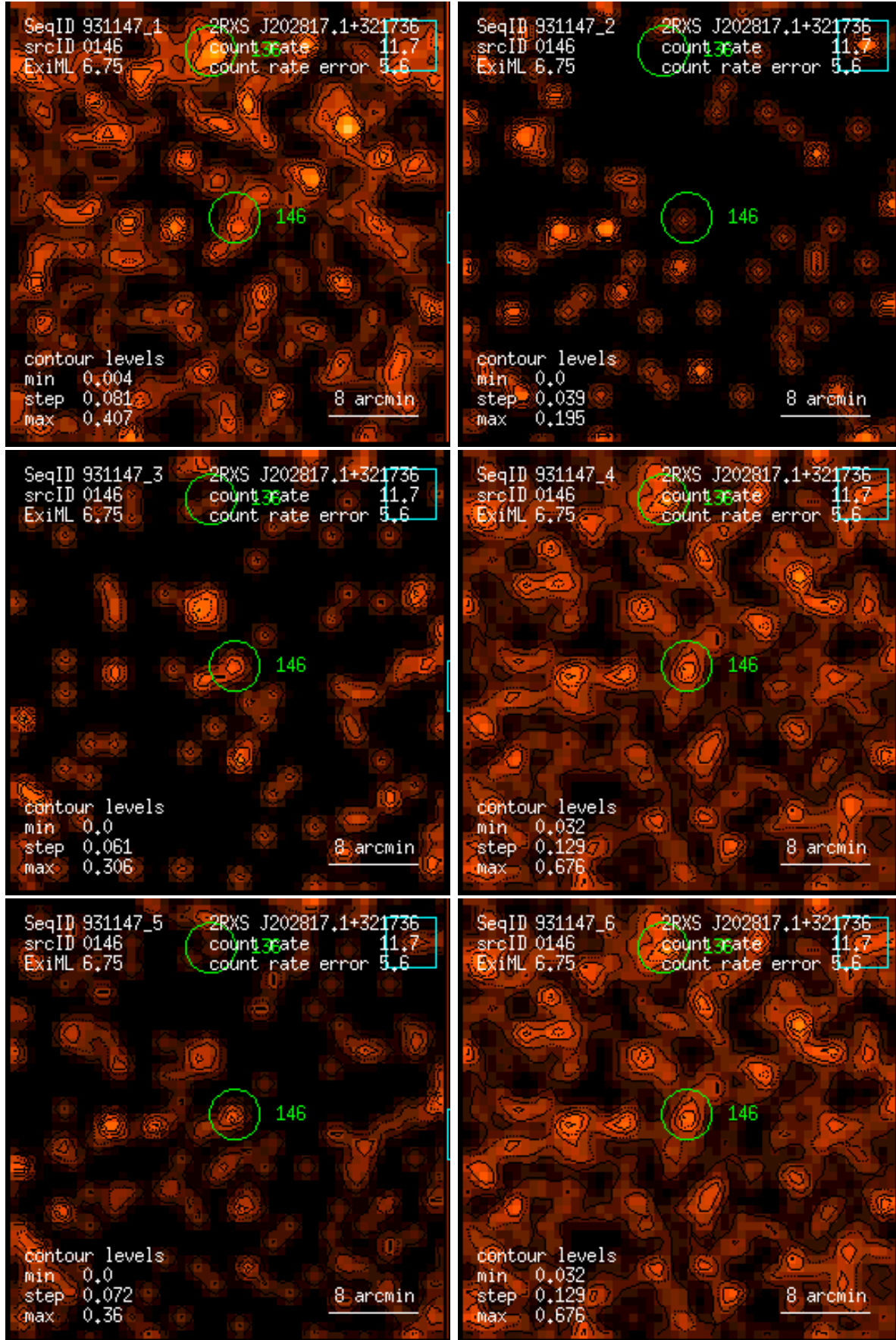
Figure 146: RASS 931147: detection 0146: band rate images, Gaussian filter: (1) PSPC channels 11 – 41, (2) 52 – 90, (3) 91 – 201, (4) 11 – 235, (5) 52 – 201, (6) 11 – 201. Broad band rates in counts/ks. Band rate contour levels in counts/ks/arcmin 2 .
