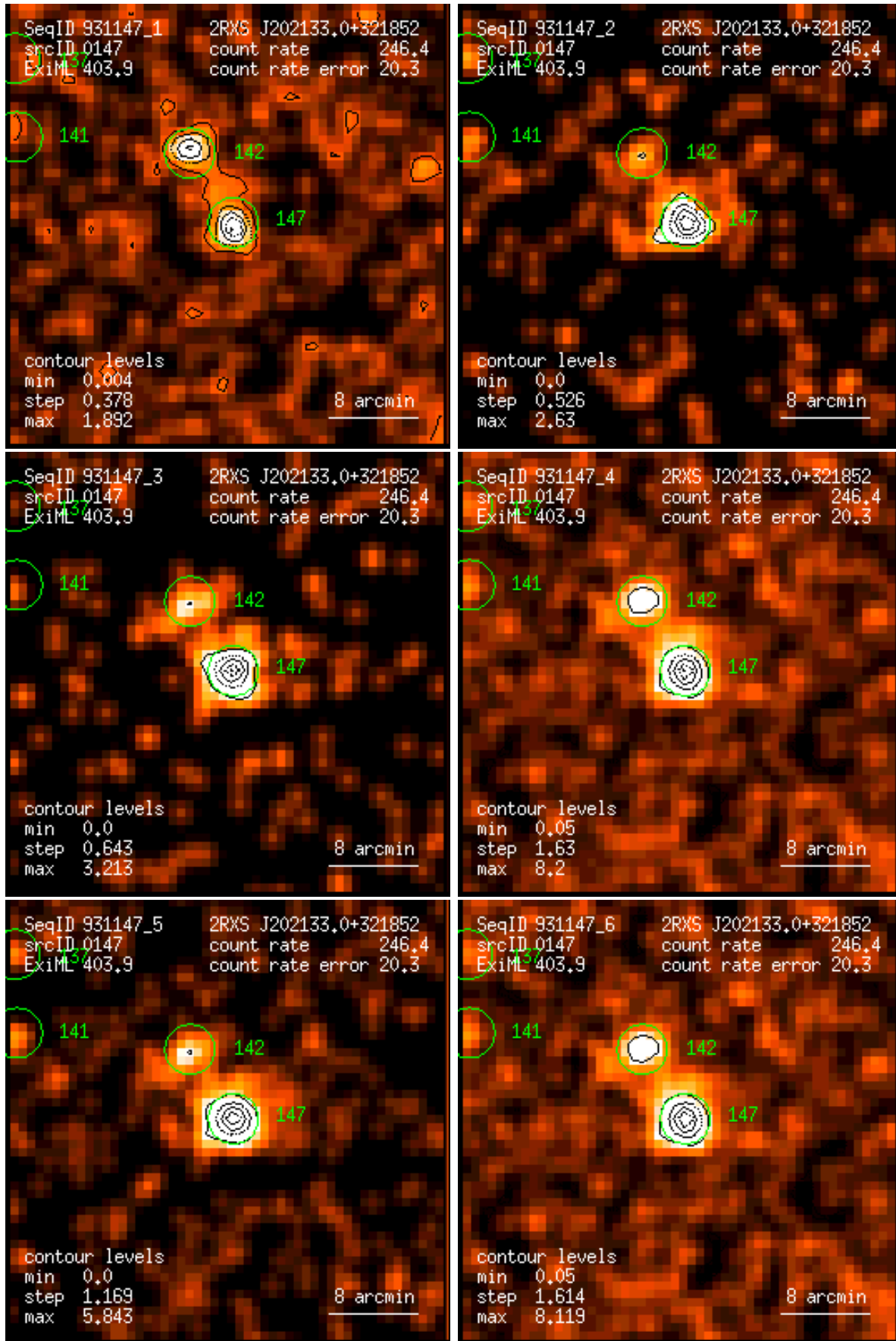
Figure 147: RASS 931147: detection 0147: band rate images, Gaussian filter: (1) PSPC channels 11 – 41, (2) 52 – 90, (3) 91 – 201, (4) 11 – 235, (5) 52 – 201, (6) 11 – 201. Broad band rates in counts/ks. Band rate contour levels in counts/ks/arcmin 2 .
