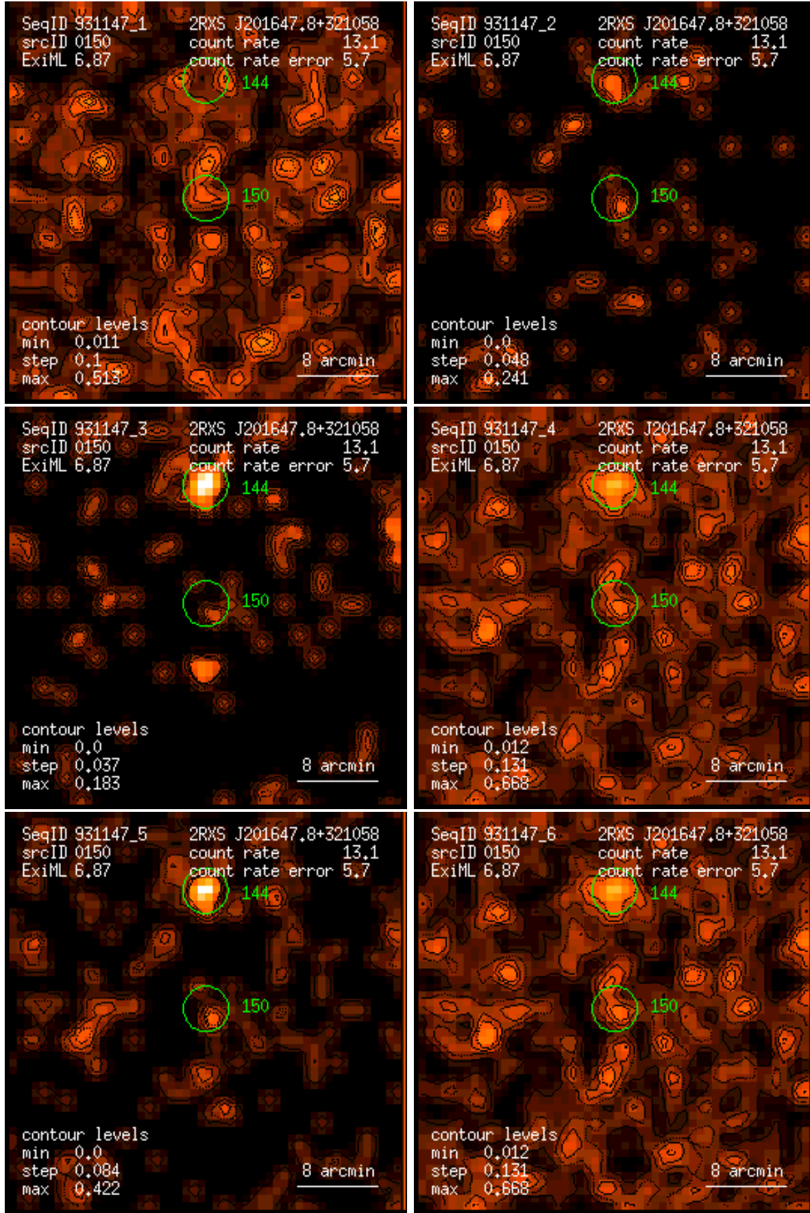
Figure 150: RASS 931147: detection 0150: band rate images, Gaussian filter: (1) PSPC channels 11 – 41, (2) 52 – 90, (3) 91 – 201, (4) 11 – 235, (5) 52 – 201, (6) 11 – 201. Broad band rates in counts/ks. Band rate contour levels in counts/ks/arcmin 2 .
