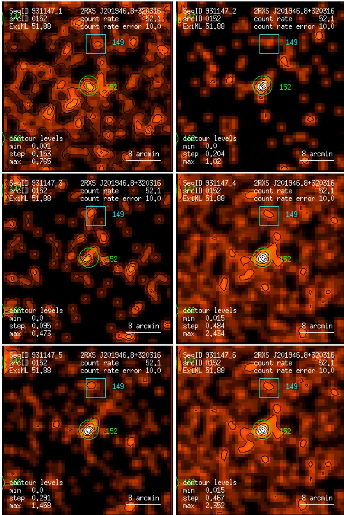
Figure 152: RASS 931147: detection 0152: band rate images, Gaussian filter: (1) PSPC channels 11 – 41, (2) 52 – 90, (3) 91 – 201, (4) 11 – 235, (5) 52 – 201, (6) 11 – 201. Broad band rates in counts/ks. Band rate contour levels in counts/ks/arcmin 2 .
