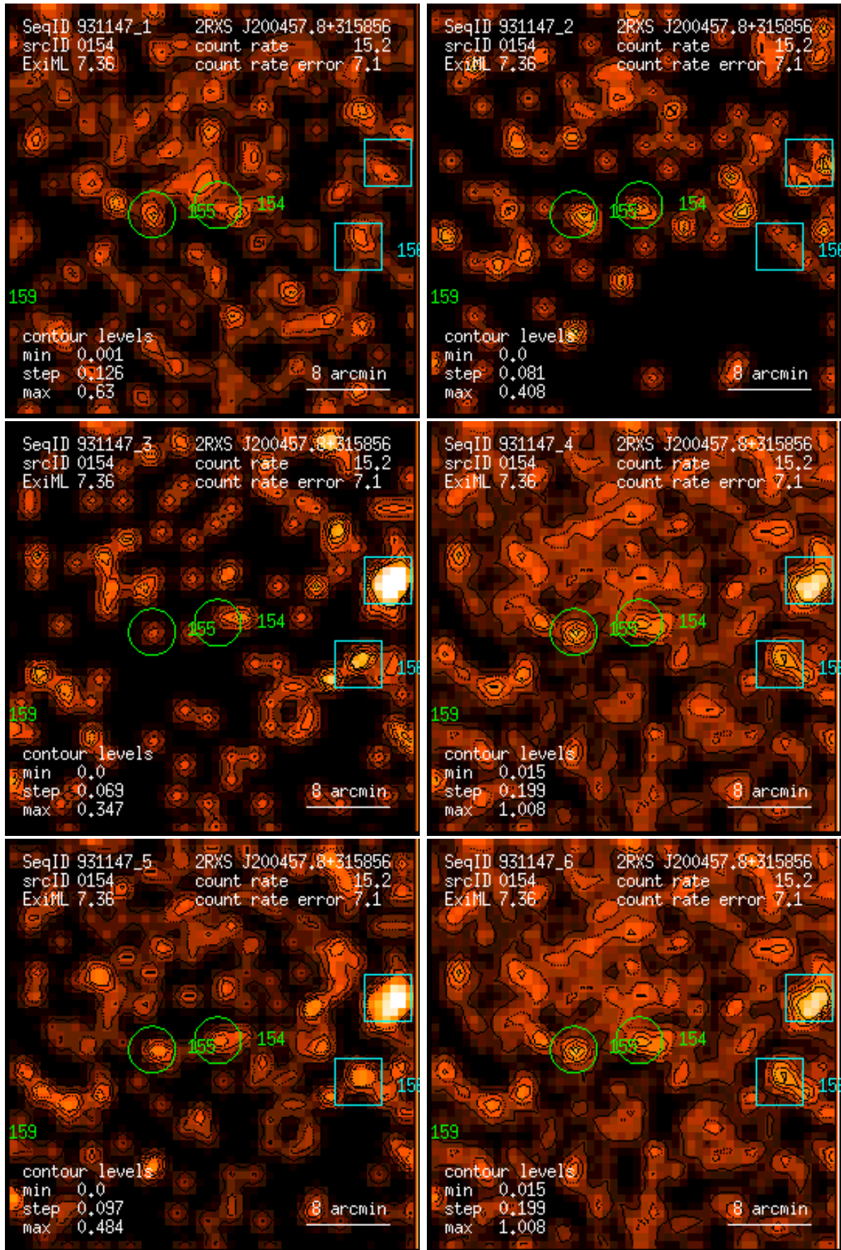
Figure 154: RASS 931147: detection 0154: band rate images, Gaussian filter: (1) PSPC channels 11 – 41, (2) 52 – 90, (3) 91 – 201, (4) 11 – 235, (5) 52 – 201, (6) 11 – 201. Broad band rates in counts/ks. Band rate contour levels in counts/ks/arcmin 2 .
