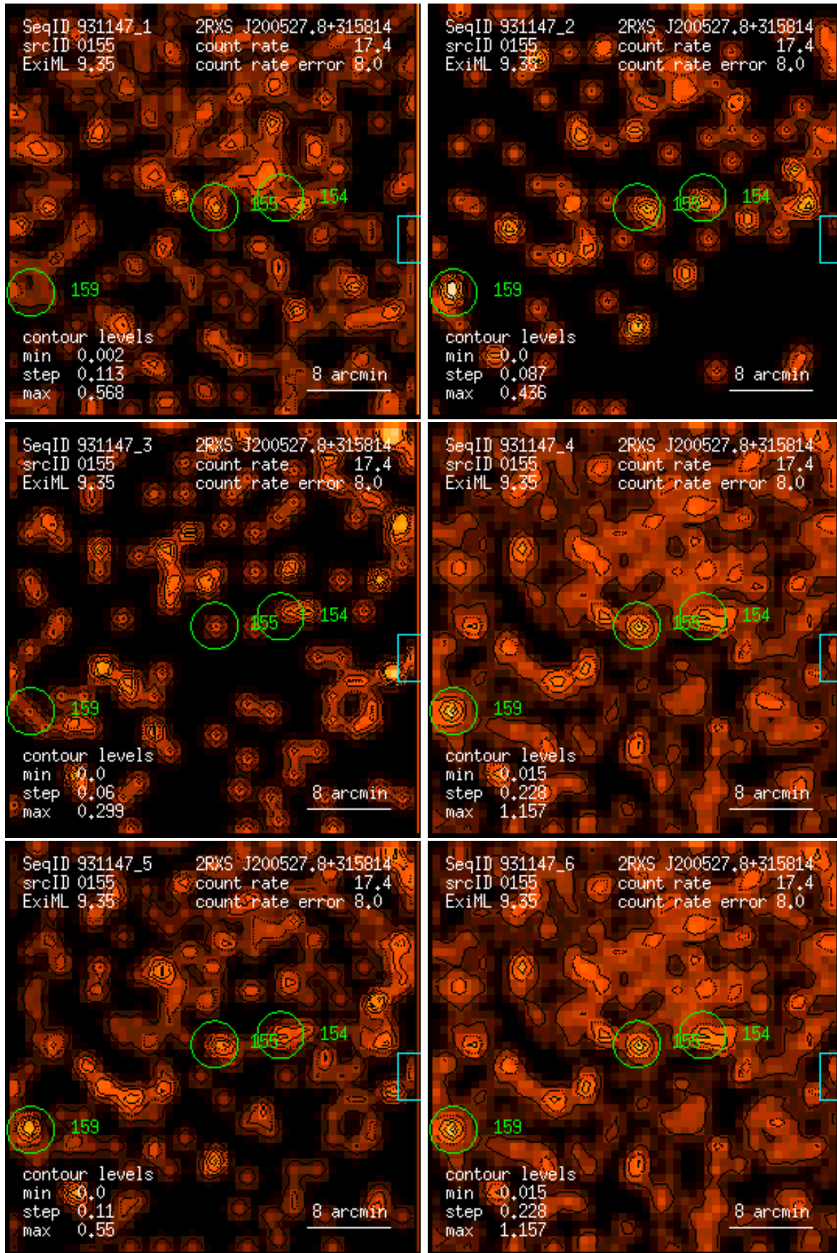
Figure 155: RASS 931147: detection 0155: band rate images, Gaussian filter: (1) PSPC channels 11 – 41, (2) 52 – 90, (3) 91 – 201, (4) 11 – 235, (5) 52 – 201, (6) 11 – 201. Broad band rates in counts/ks. Band rate contour levels in counts/ks/arcmin 2 .
