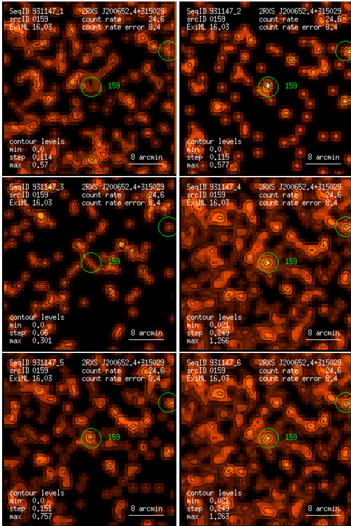
Figure 159: RASS 931147: detection 0159: band rate images, Gaussian filter: (1) PSPC channels 11 – 41, (2) 52 – 90, (3) 91 – 201, (4) 11 – 235, (5) 52 – 201, (6) 11 – 201. Broad band rates in counts/ks. Band rate contour levels in counts/ks/arcmin 2 .
