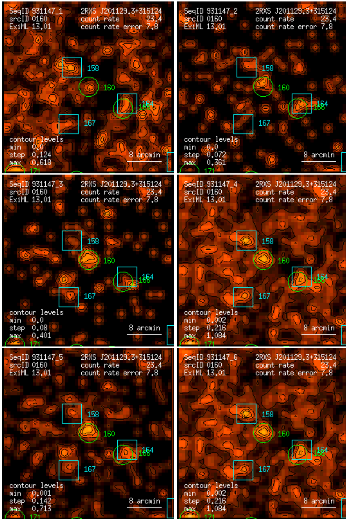
Figure 160: RASS 931147: detection 0160: band rate images, Gaussian filter: (1) PSPC channels 11 – 41, (2) 52 – 90, (3) 91 – 201, (4) 11 – 235, (5) 52 – 201, (6) 11 – 201. Broad band rates in counts/ks. Band rate contour levels in counts/ks/arcmin 2 .
