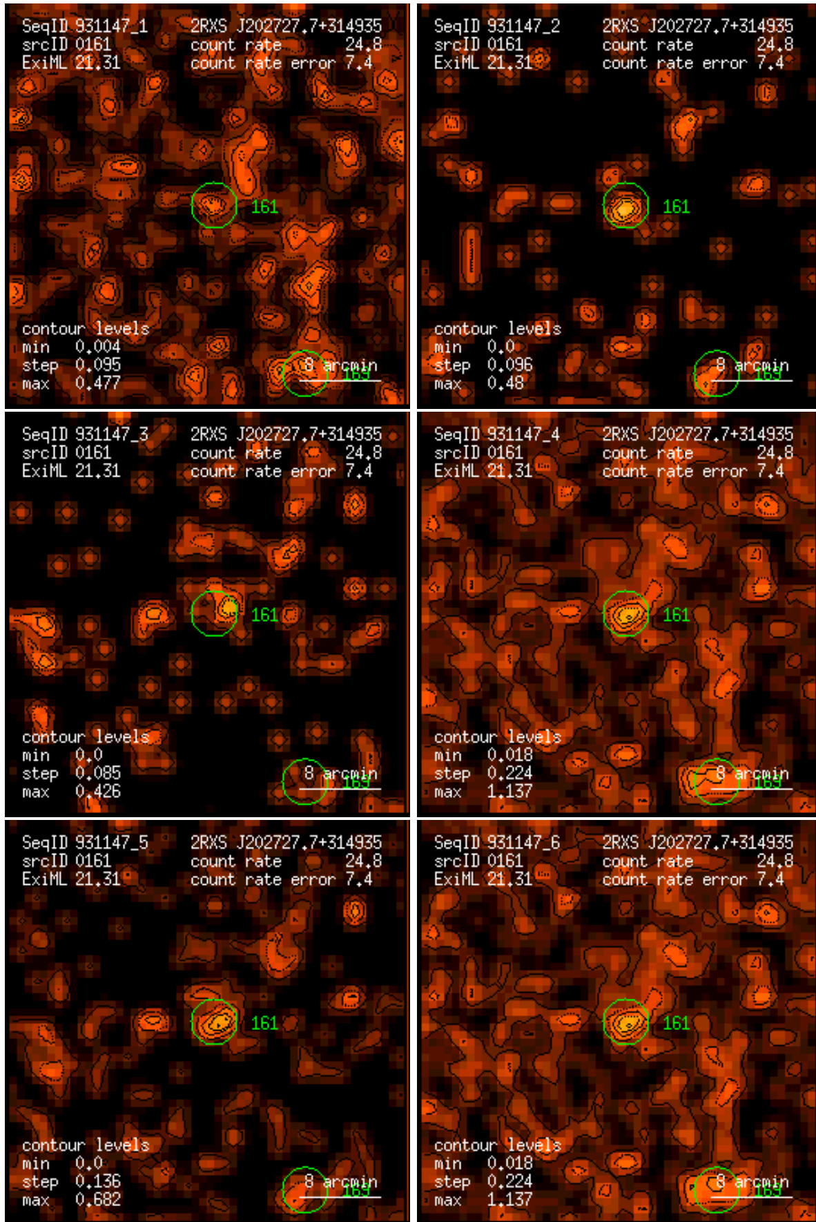
Figure 161: RASS 931147: detection 0161: band rate images, Gaussian filter: (1) PSPC channels 11 – 41, (2) 52 – 90, (3) 91 – 201, (4) 11 – 235, (5) 52 – 201, (6) 11 – 201. Broad band rates in counts/ks. Band rate contour levels in counts/ks/arcmin 2 .
