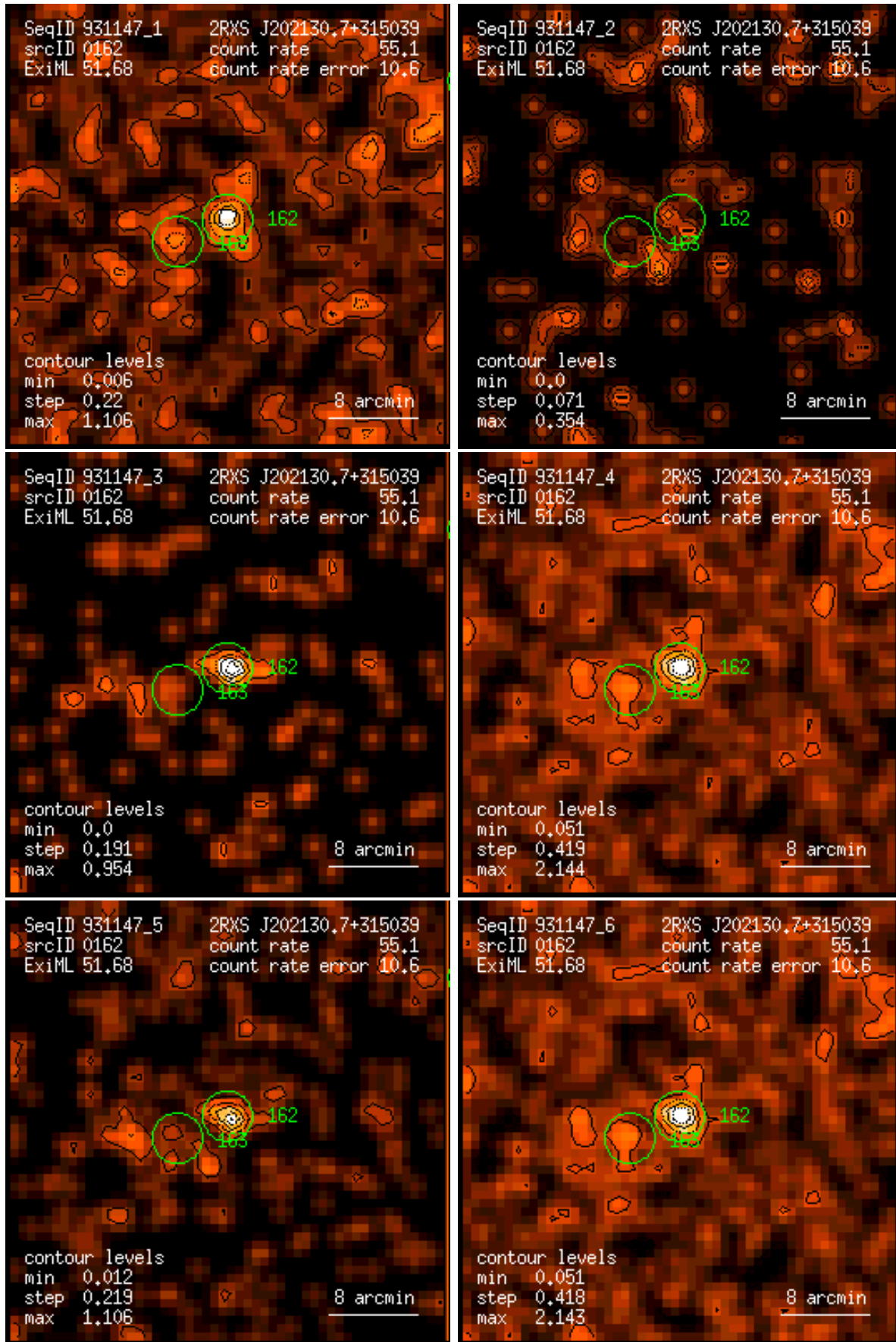
Figure 162: RASS 931147: detection 0162: band rate images, Gaussian filter: (1) PSPC channels 11 – 41, (2) 52 – 90, (3) 91 – 201, (4) 11 – 235, (5) 52 – 201, (6) 11 – 201. Broad band rates in counts/ks. Band rate contour levels in counts/ks/arcmin 2 .
