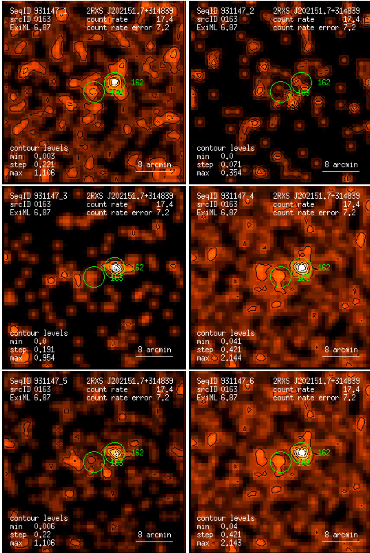
Figure 163: RASS 931147: detection 0163: band rate images, Gaussian filter: (1) PSPC channels 11 – 41, (2) 52 – 90, (3) 91 – 201, (4) 11 – 235, (5) 52 – 201, (6) 11 – 201. Broad band rates in counts/ks. Band rate contour levels in counts/ks/arcmin 2 .
