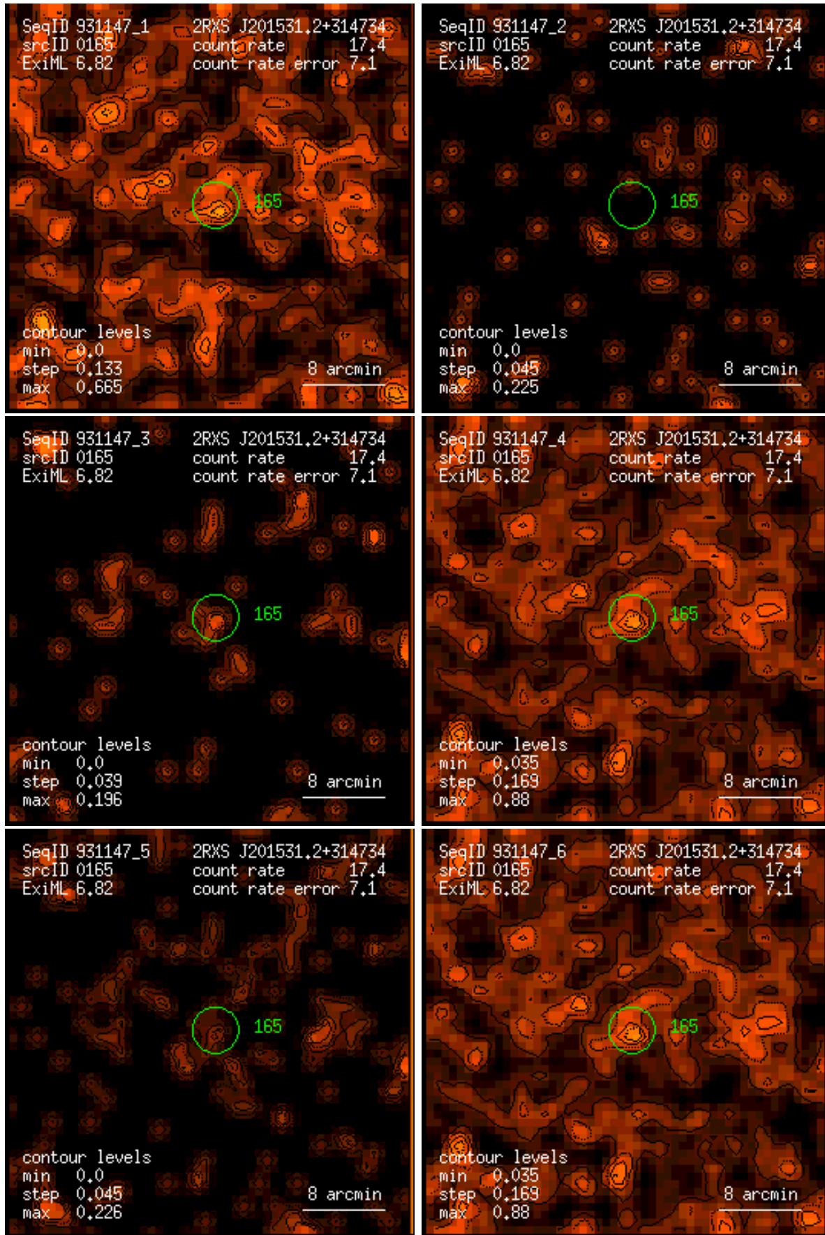
Figure 165: RASS 931147: detection 0165: band rate images, Gaussian filter: (1) PSPC channels 11 – 41, (2) 52 – 90, (3) 91 – 201, (4) 11 – 235, (5) 52 – 201, (6) 11 – 201. Broad band rates in counts/ks. Band rate contour levels in counts/ks/arcmin 2 .
