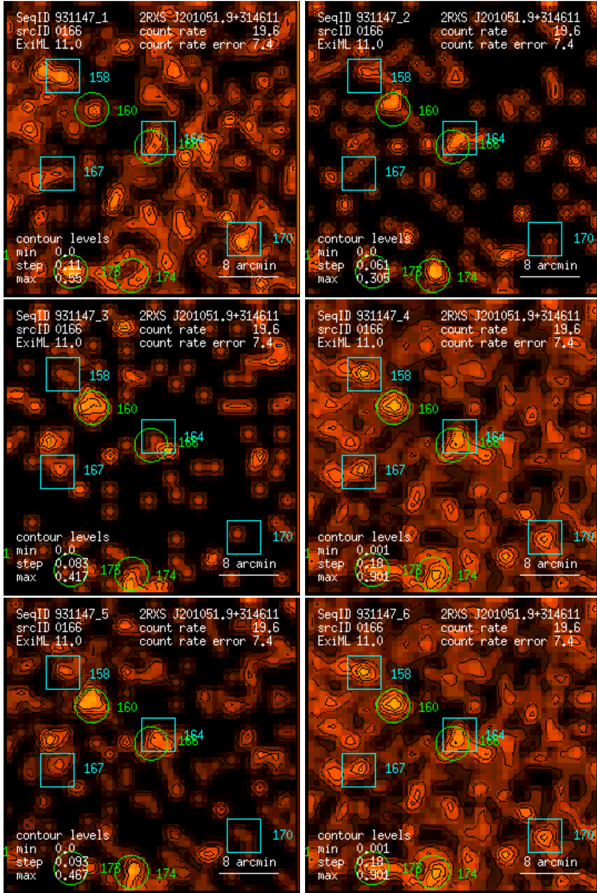
Figure 166: RASS 931147: detection 0166: band rate images, Gaussian filter: (1) PSPC channels 11 – 41, (2) 52 – 90, (3) 91 – 201, (4) 11 – 235, (5) 52 – 201, (6) 11 – 201. Broad band rates in counts/ks. Band rate contour levels in counts/ks/arcmin 2 .
