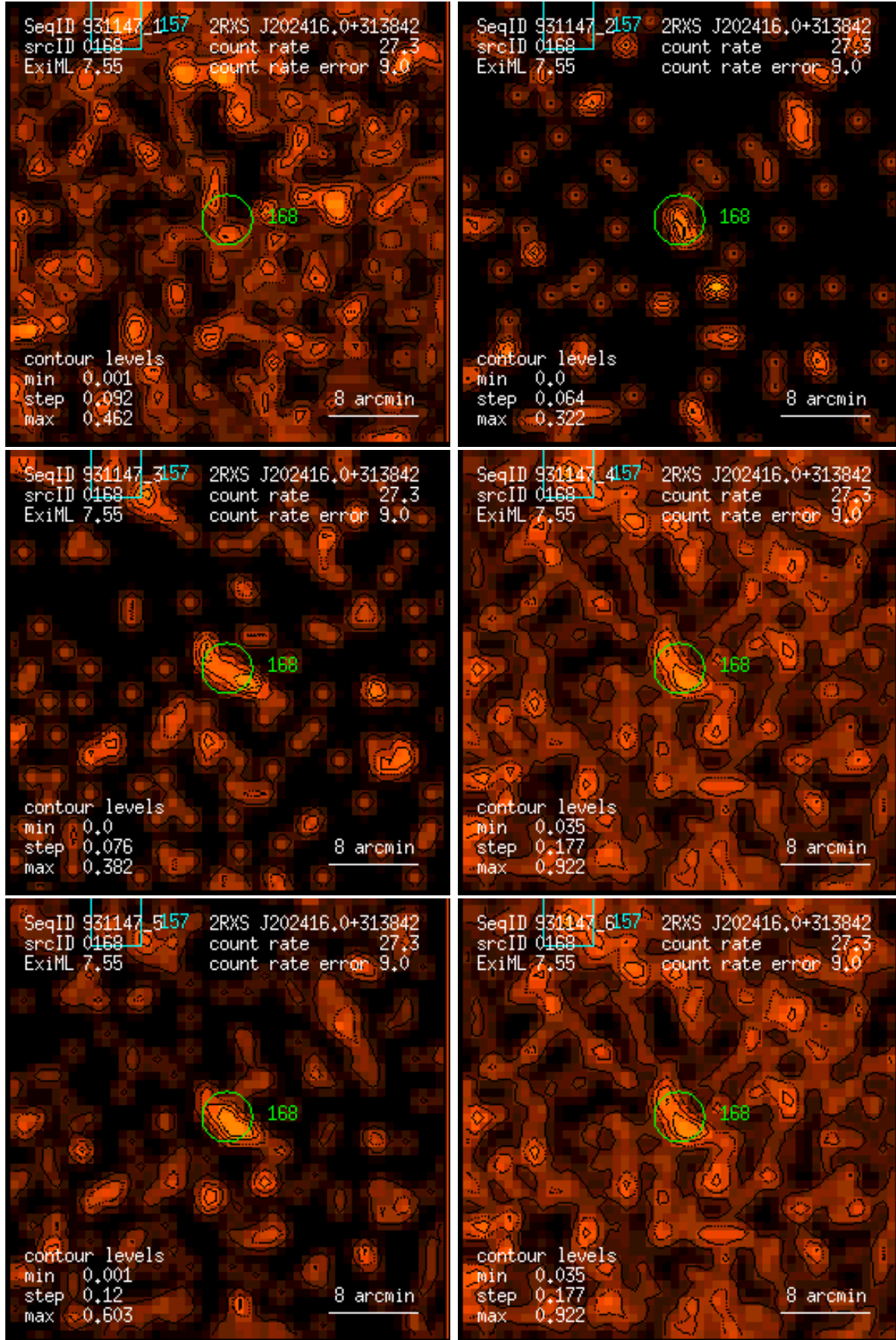
Figure 168: RASS 931147: detection 0168: band rate images, Gaussian filter: (1) PSPC channels 11 – 41, (2) 52 – 90, (3) 91 – 201, (4) 11 – 235, (5) 52 – 201, (6) 11 – 201. Broad band rates in counts/ks. Band rate contour levels in counts/ks/arcmin 2 .
