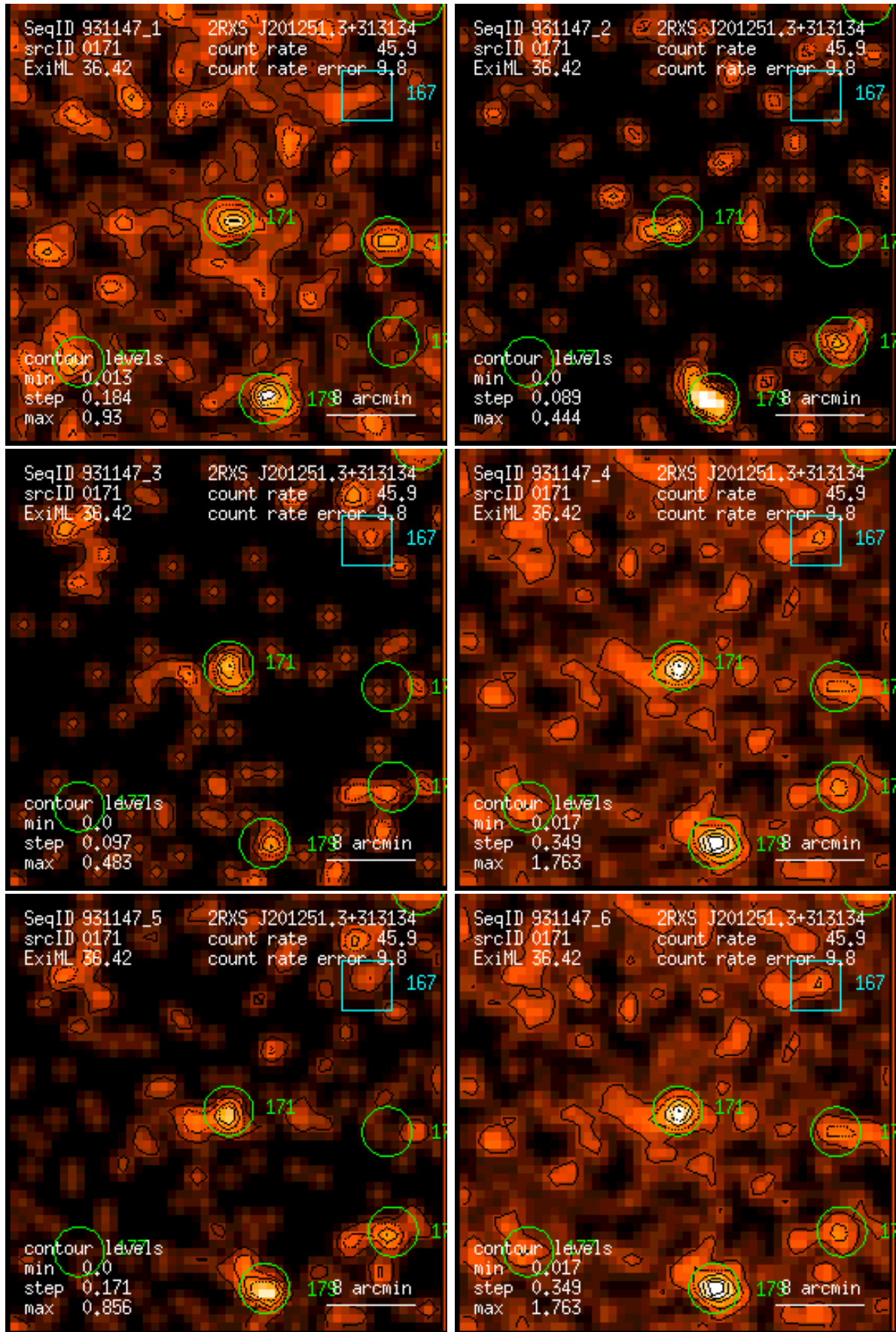
Figure 171: RASS 931147: detection 0171: band rate images, Gaussian filter: (1) PSPC channels 11 – 41, (2) 52 – 90, (3) 91 – 201, (4) 11 – 235, (5) 52 – 201, (6) 11 – 201. Broad band rates in counts/ks. Band rate contour levels in counts/ks/arcmin 2 .
