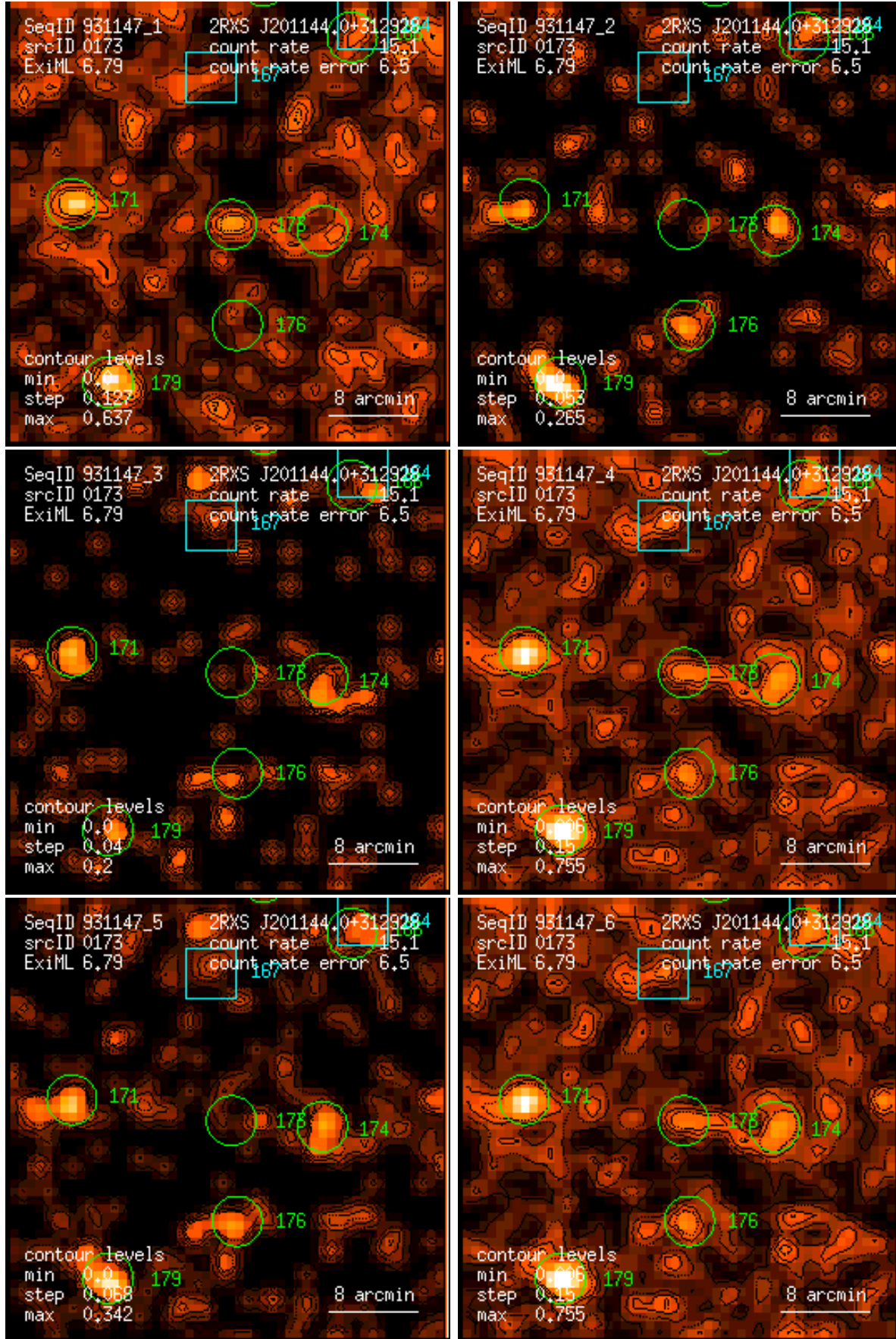
Figure 173: RASS 931147: detection 0173: band rate images, Gaussian filter: (1) PSPC channels 11 – 41, (2) 52 – 90, (3) 91 – 201, (4) 11 – 235, (5) 52 – 201, (6) 11 – 201. Broad band rates in counts/ks. Band rate contour levels in counts/ks/arcmin 2 .
