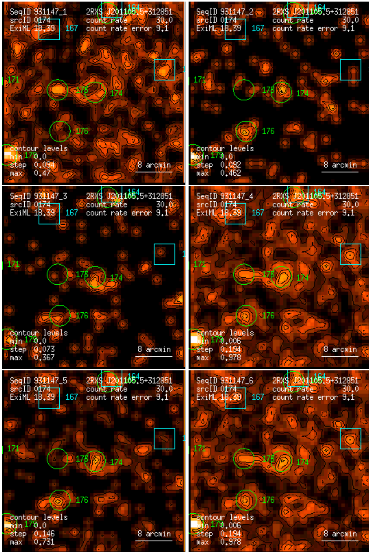
Figure 174: RASS 931147: detection 0174: band rate images, Gaussian filter: (1) PSPC channels 11 – 41, (2) 52 – 90, (3) 91 – 201, (4) 11 – 235, (5) 52 – 201, (6) 11 – 201. Broad band rates in counts/ks. Band rate contour levels in counts/ks/arcmin 2 .
