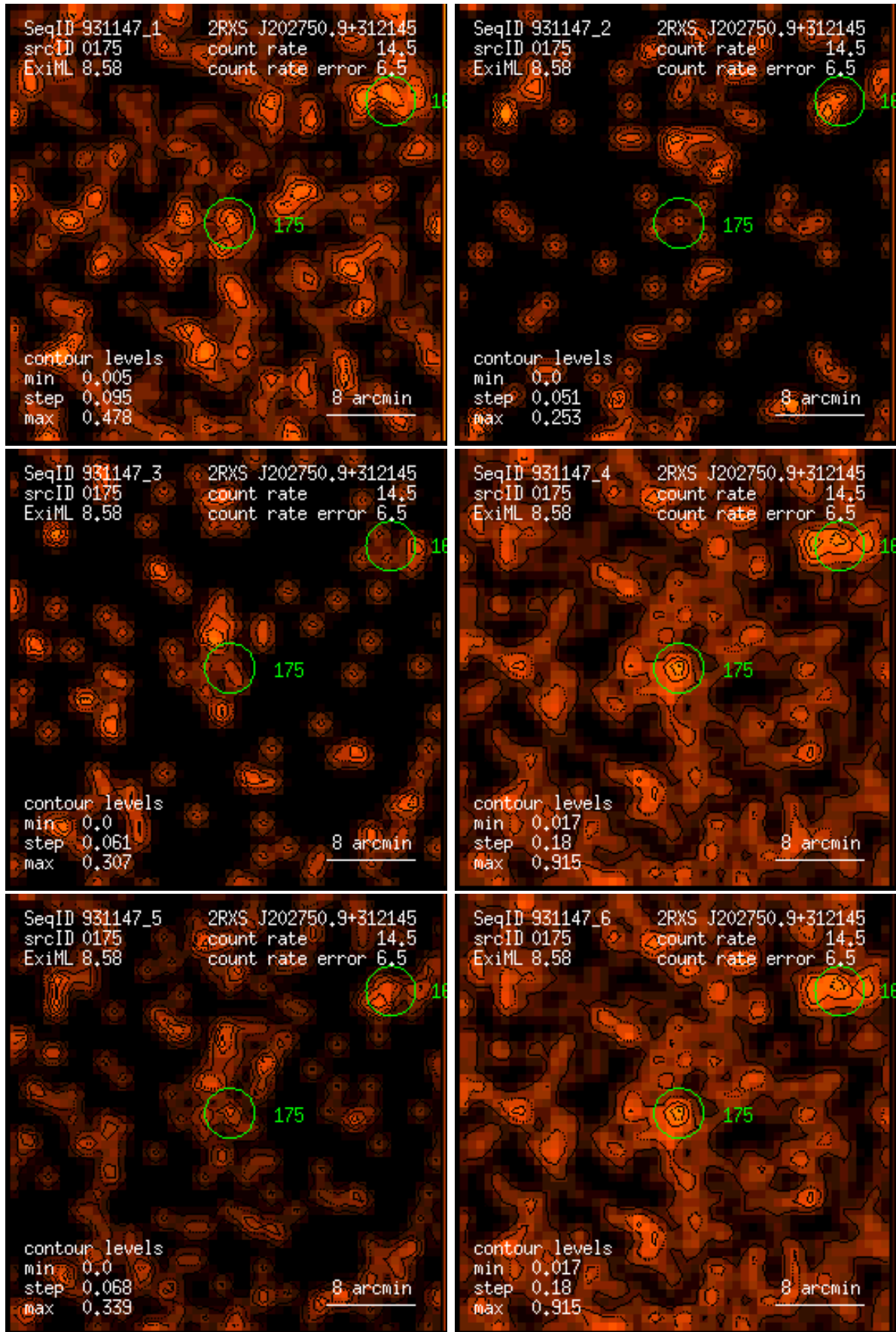
Figure 175: RASS 931147: detection 0175: band rate images, Gaussian filter: (1) PSPC channels 11 – 41, (2) 52 – 90, (3) 91 – 201, (4) 11 – 235, (5) 52 – 201, (6) 11 – 201. Broad band rates in counts/ks. Band rate contour levels in counts/ks/arcmin 2 .
