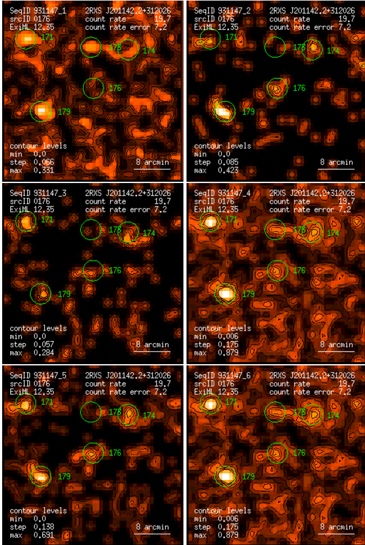
Figure 176: RASS 931147: detection 0176: band rate images, Gaussian filter: (1) PSPC channels 11 – 41, (2) 52 – 90, (3) 91 – 201, (4) 11 – 235, (5) 52 – 201, (6) 11 – 201. Broad band rates in counts/ks. Band rate contour levels in counts/ks/arcmin 2 .
