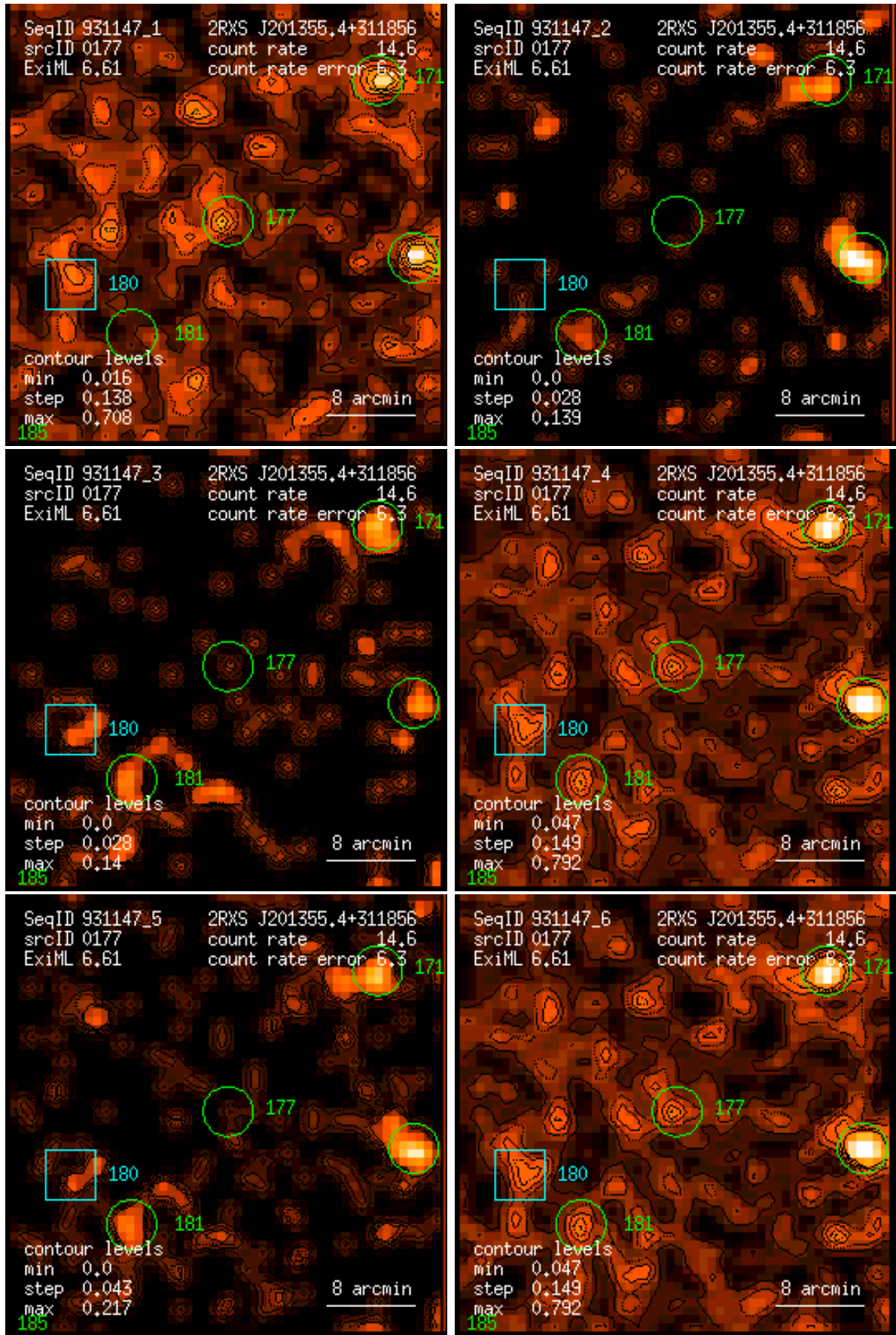
Figure 177: RASS 931147: detection 0177: band rate images, Gaussian filter: (1) PSPC channels 11 – 41, (2) 52 – 90, (3) 91 – 201, (4) 11 – 235, (5) 52 – 201, (6) 11 – 201. Broad band rates in counts/ks. Band rate contour levels in counts/ks/arcmin 2 .
